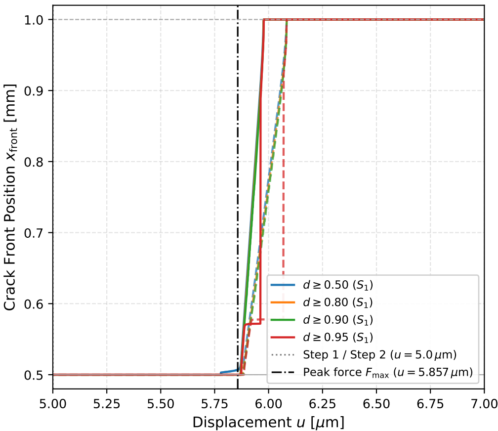
(a) Continuous Crack Front x_{\text{front}}(u)
