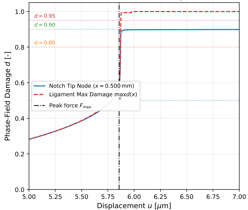
(c) Notch-Root Saturation Physics
