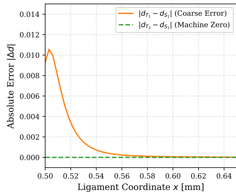
Pointwise Error at Peak F_{\max} ( u = 0.005857 mm)
