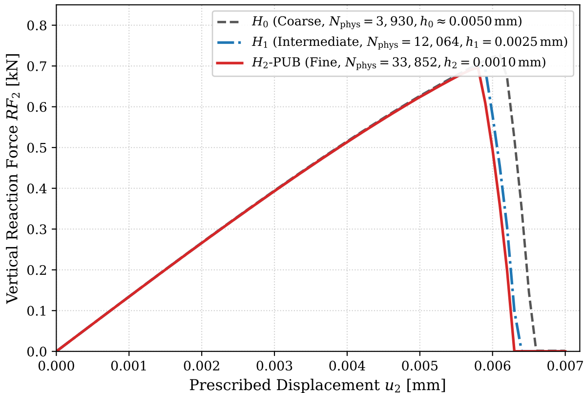
Uniform Mesh Convergence: Mode-I Tension ( \ell_0 = 0.015 mm)
