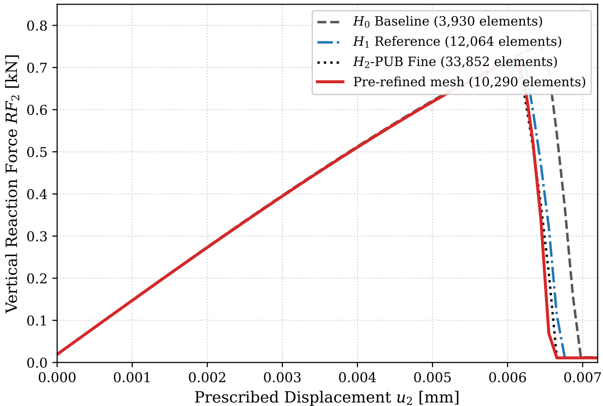
Force--Displacement Comparison: Pre-Refined vs. Uniform Meshes
