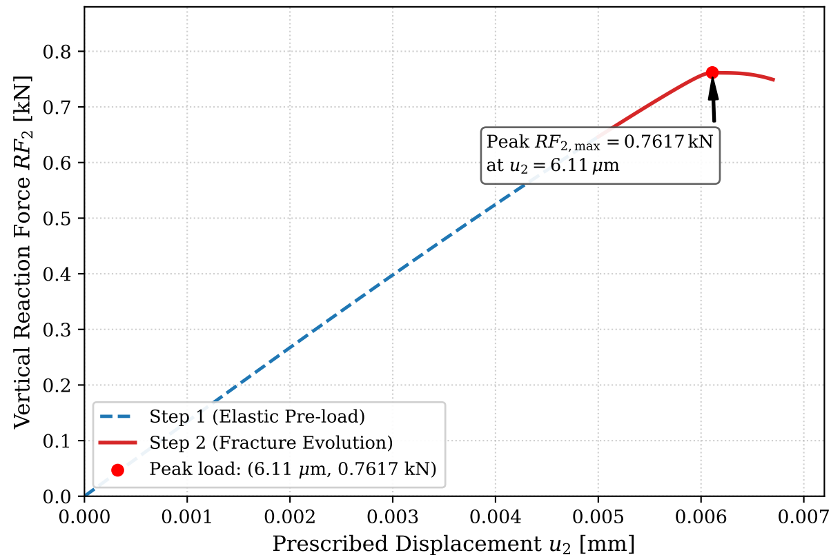
Molnar Single-Edge-Notched Tension ( \ell_0 = 0.0075 mm)
