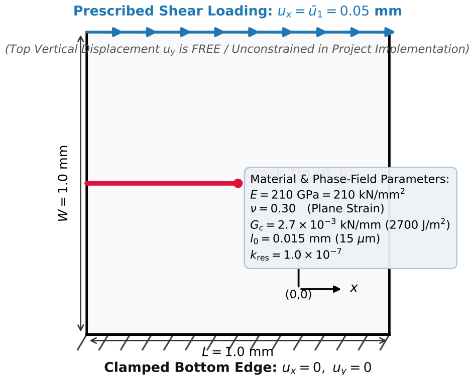
Figure 1: Mode-II Single-Edge-Notched Plate Benchmark Specification
