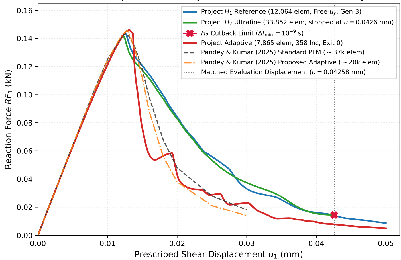
Figure 5: Mode-II Force-Displacement Response: Fixed References vs Adaptive vs Literature
