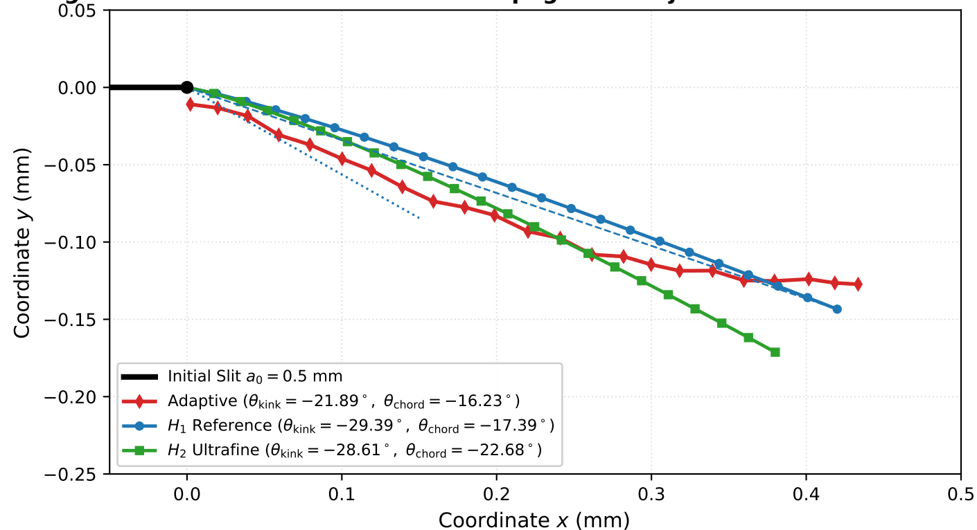
Figure 9: Extracted Mode-II Crack Propagation Trajectories & Kinematic Angles
