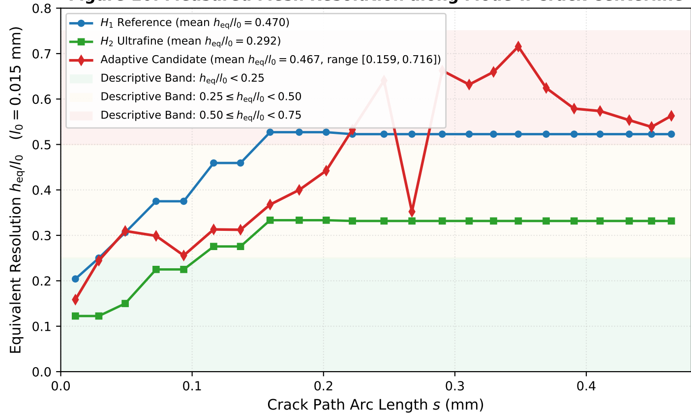
Figure 10: Measured Mesh Resolution along Mode-II Crack Centerline
