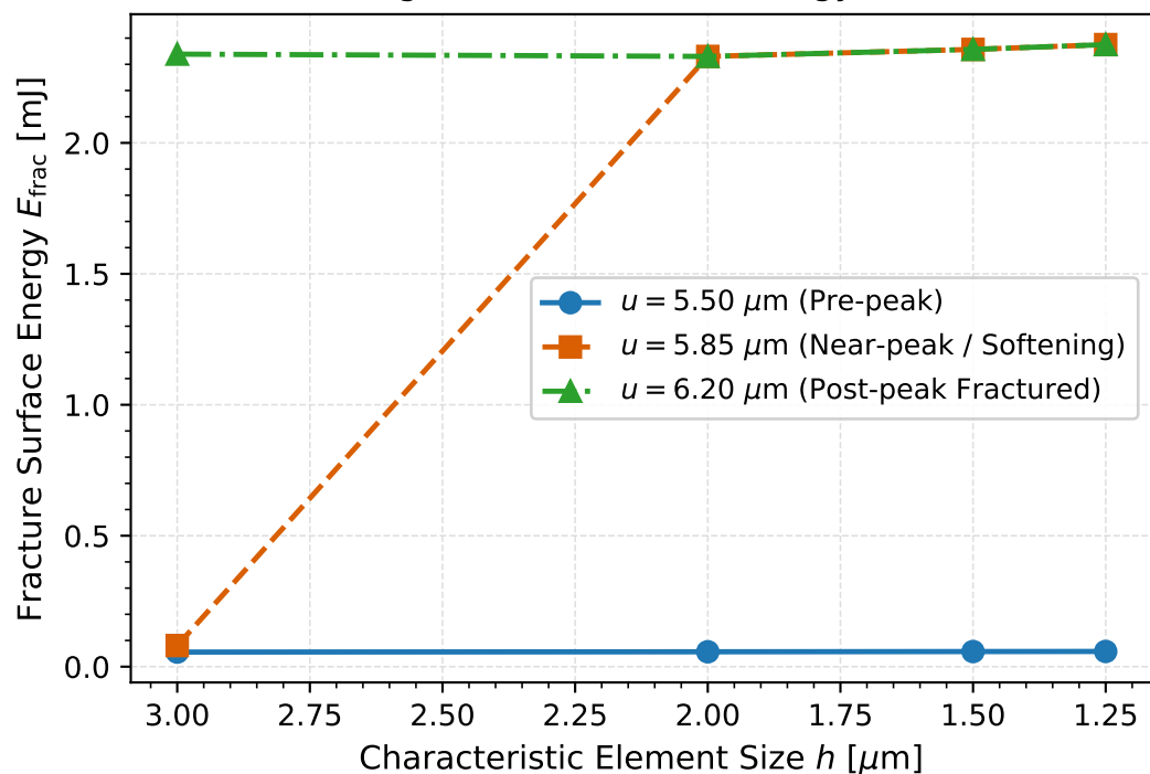
(c) Regularized Fracture Energy E_{\text{frac}}(u)
