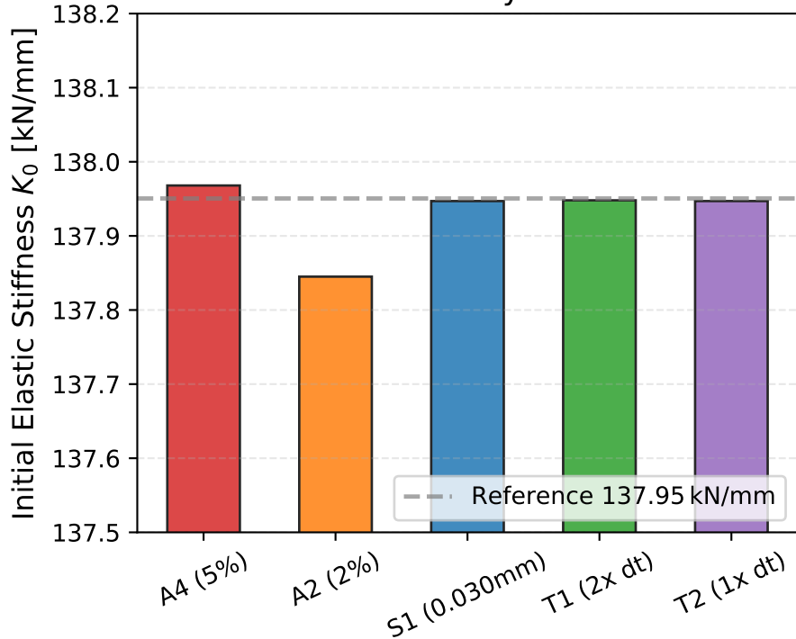
Elastic Stiffness Parity across Meshes
