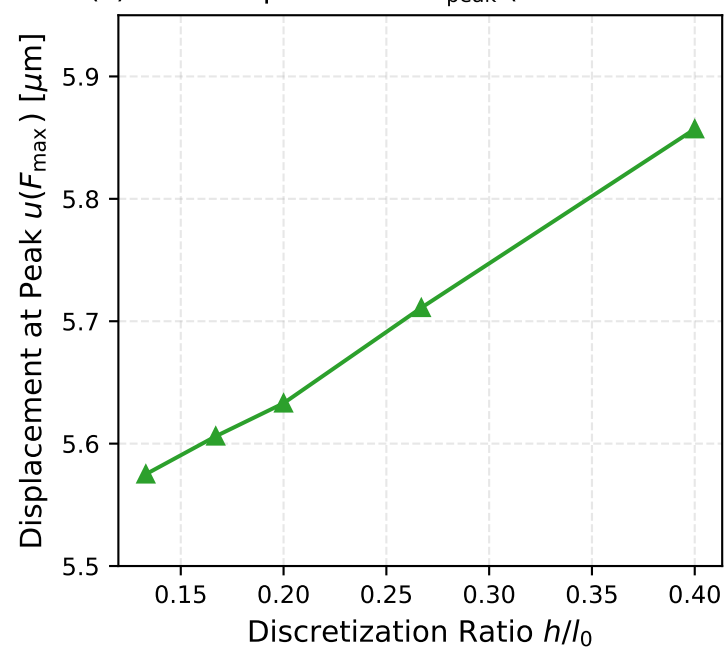
(c) Peak Displacement u_{\text{peak}} (Mesh-Sensitive)
