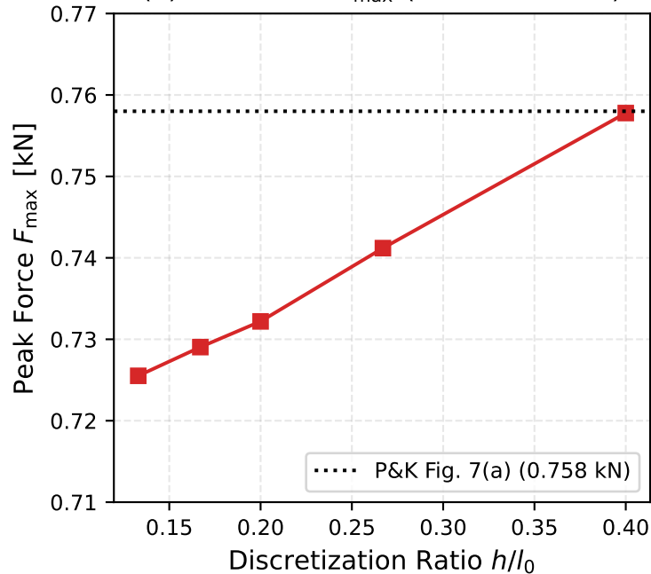
(b) Peak Force F_{\max} (Mesh-Sensitive)
