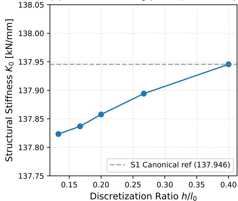
(a) Initial Stiffness K_0 (Stable, \Delta < 0.09\% )
