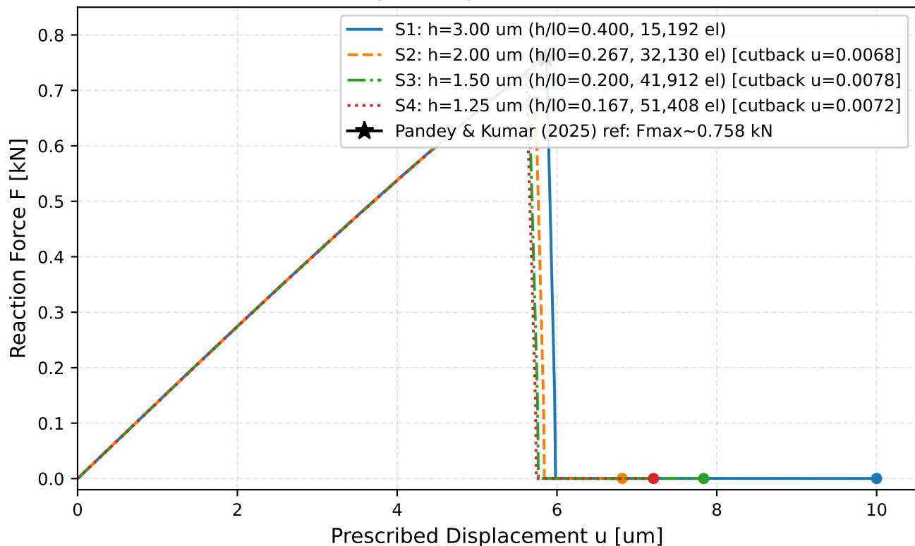
Mode-I Tensile Response: Spatial Fixed-Mesh Series (S1--S4)
