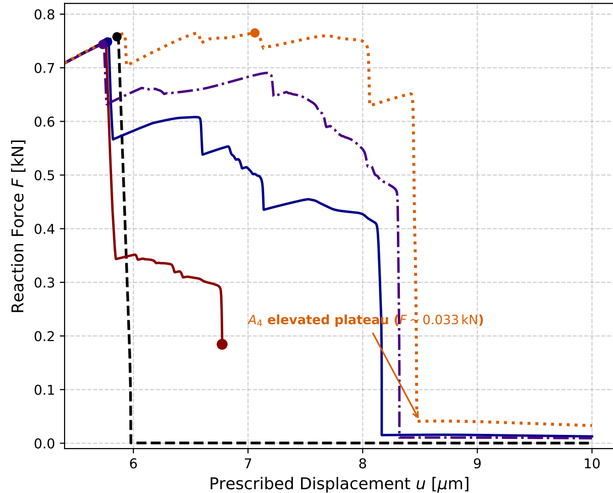
(b) Post-Peak & Softening Zoom ( u \geq 5.4\mu\text{m} )
