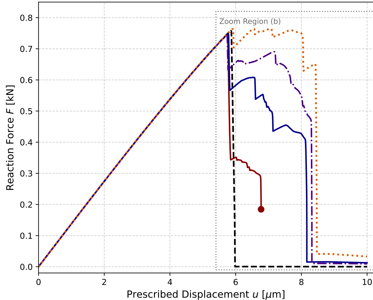
(a) Full Force--Displacement Response
