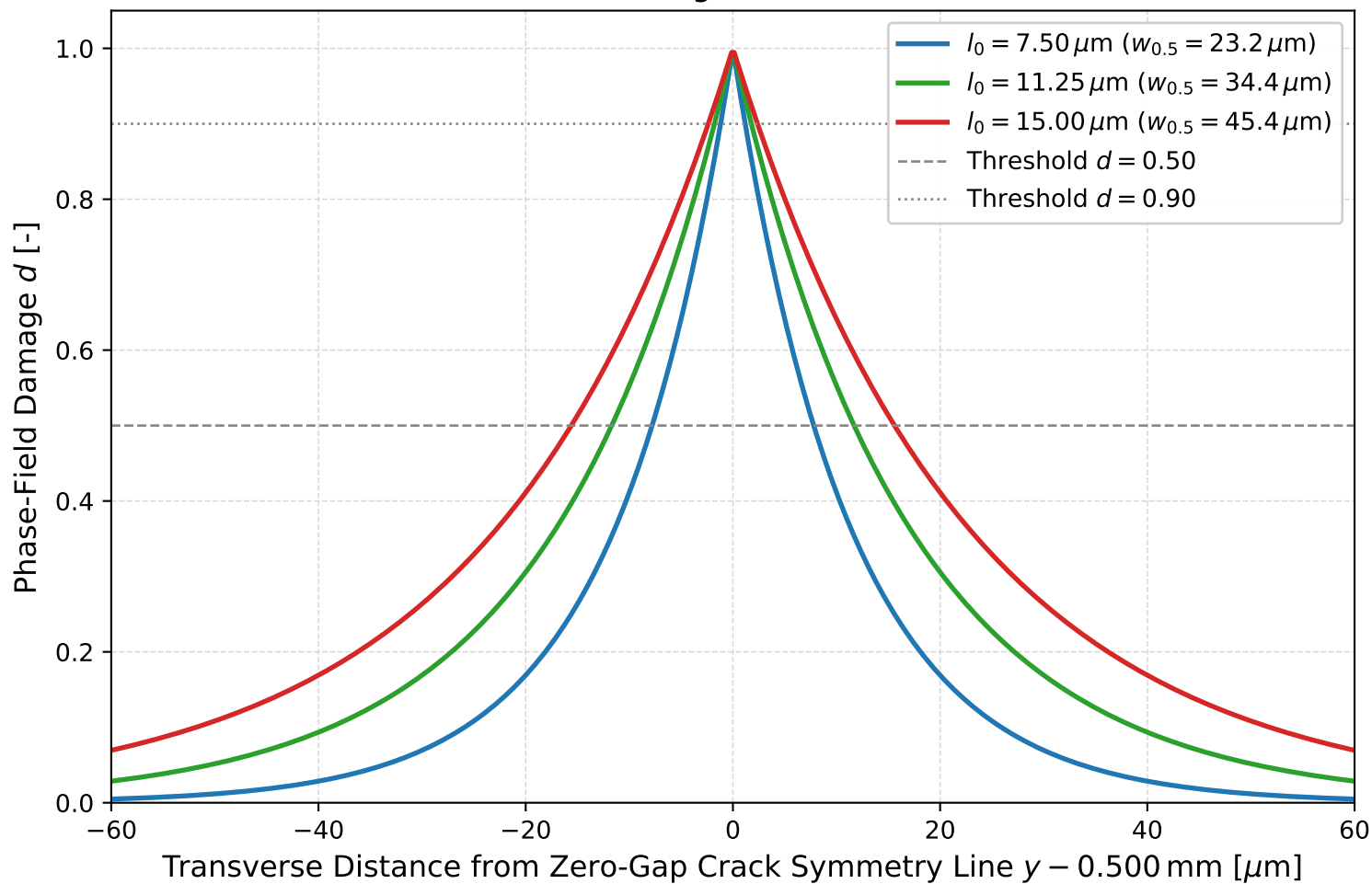
Transverse Localization Damage Profiles at Station x = 0.550 mm
