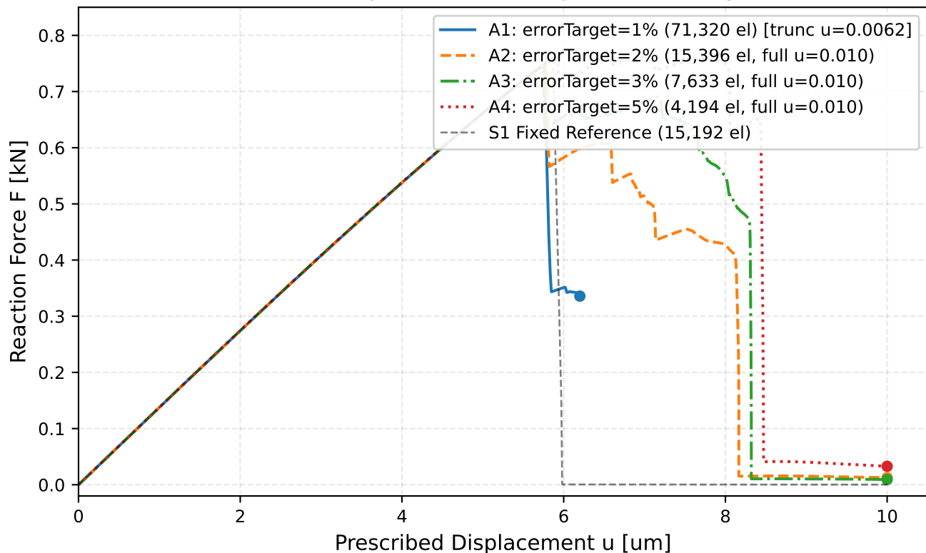
Mode-I Tensile Response: Native Adaptive Remeshing (A1--A4)
