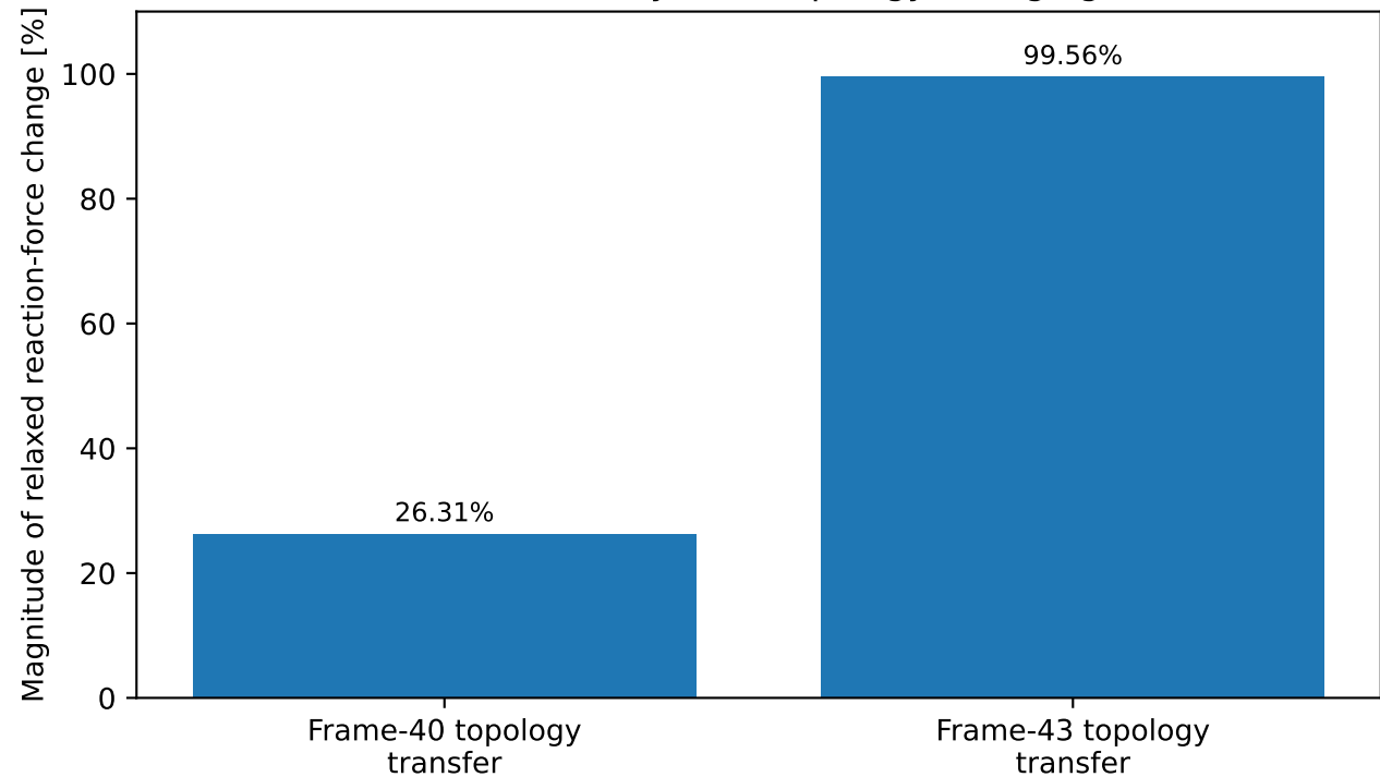
Mechanical continuity after topology-changing restart
