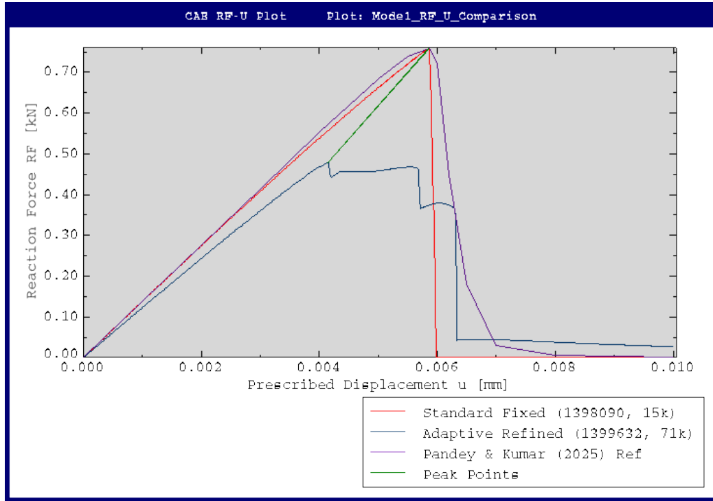
Figure 7.2: Reaction force versus prescribed displacement comparison for the Pandey & Kumar Mode-I tensile benchmark, comparing the reference curve, the accepted standard fixed mesh (1398090.mmaste02), and the completed sharp-slit adaptive calculation (1399632.mmaste02).
