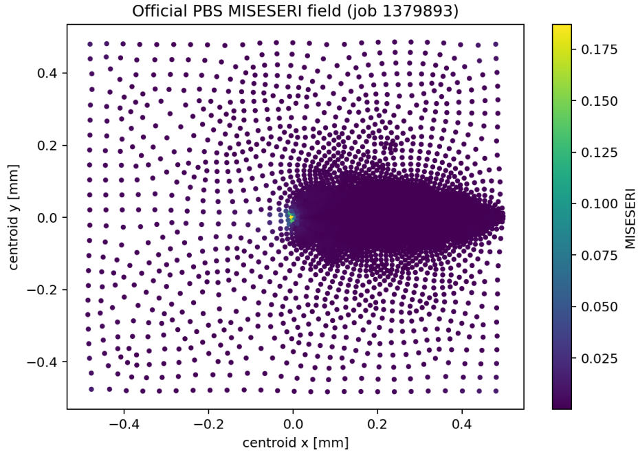
Figure 3.1: Spatial distribution of the official PBS-extracted MisesERI field from coarse pre-analysis job 1379893.mm master02 . The plot is generated from the 3,930-row extraction CSV with SHA-256 49b0c5f7a784f361...; the ODB, CSV and repaired validation are recorded together in the Stage-F4 replacement evidence. This is a derived plot of Abaqus element-field output, not a reconstructed phase-field contour.
