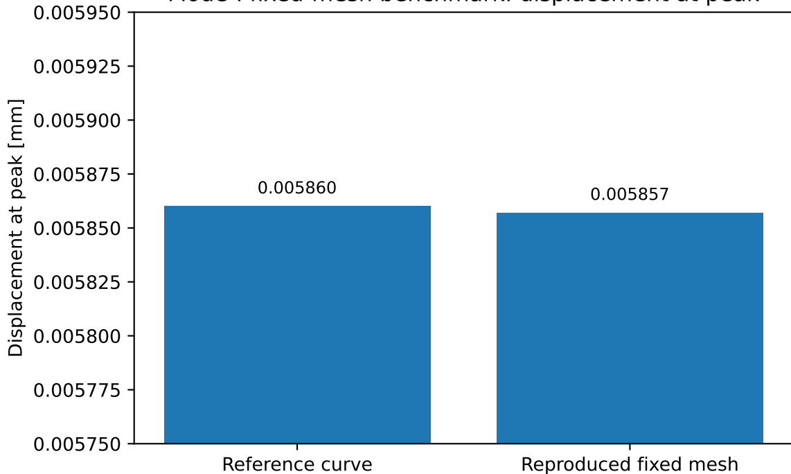
Mode-I fixed-mesh benchmark: displacement at peak
