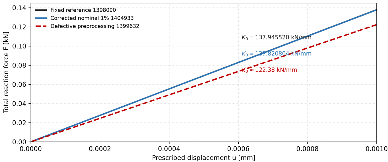
Figure 6: Initial elastic-range zoom. The corrected model and fixed reference overlap near 138 kN/mm; the defective branch remains near 122.38 kN/mm.
