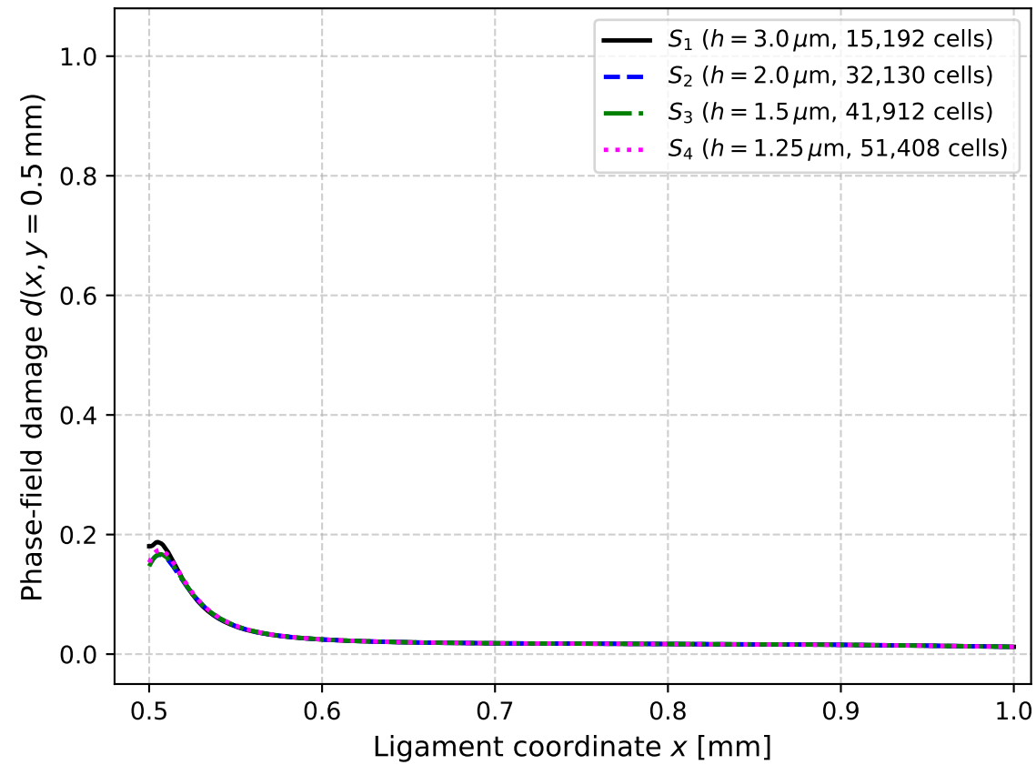
(b) Pre-Peak: u = 5.50 \mu\text{m}
