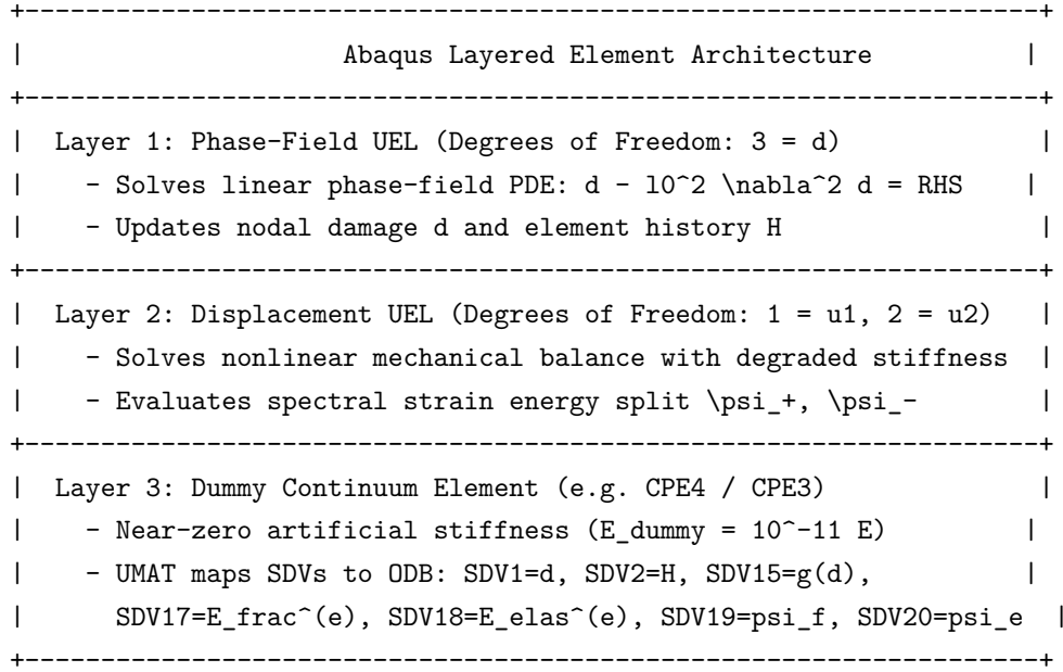
Figure 1.1: Schematic representation of the layered user-element (UEL/UMAT) architecture in Abaqus.
