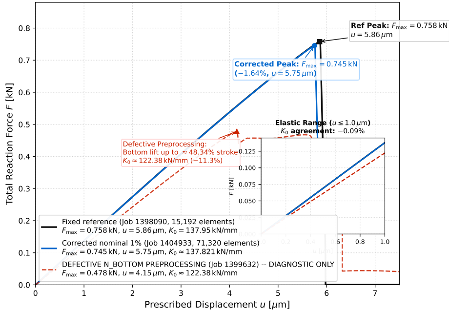
Figure 3.7: Force–displacement response demonstrating reference-consistent structural stiffness recovery (within 0.09%) upon correcting the N_BOTTOM card format.
