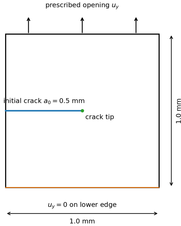
Figure 2.1: Mode-I benchmark boundary value problem: 1.0 \text{ mm} \times 1.0 \text{ mm} square domain with a sharp edge crack of length a_0 = 0.5 \text{ mm} along y = 0.5 \text{ mm} . Boundary conditions enforce roller support ( u_y = 0 ) on the bottom edge with a pinned point ( u_x = 0 ) to eliminate rigid-body motion, and uniform tensile displacement u_y = u on the top edge.
