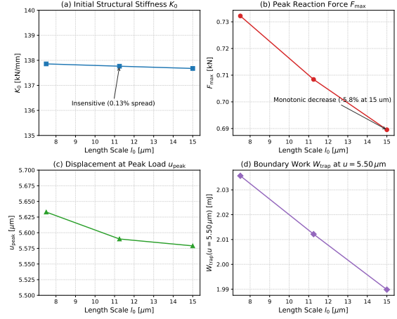
(b) Peak metrics vs. l_0
