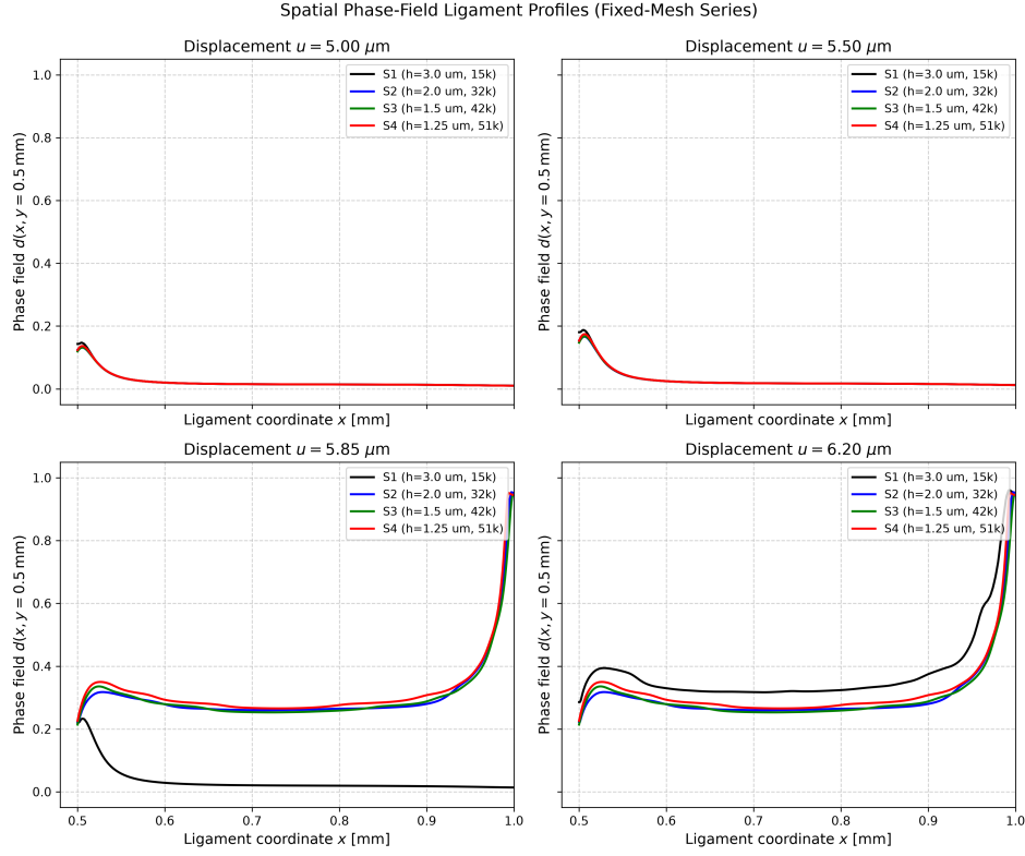
Figure 7.7: Ligament phase-field profiles d(x, y = 0.5 \text{ mm}) for fixed meshes at matched displacement increments.
