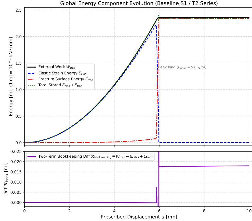
Figure 7.9: Global energy component evolution for the baseline S_1/T_2 trajectory (15,192 elements). The two-term bookkeeping difference remains within \pm 0.008\% over the specifically qualified pre-peak S_1/T_1 – T_3 trajectories. In the post-peak regime it reaches +0.7607\% for S_1/T_2 . This quantity is an endpoint bookkeeping difference and is not interpreted as an energy residual or conservation error. GLOBAL_ENERGY_IDENTITY -- NOT_YET_CLOSED.
