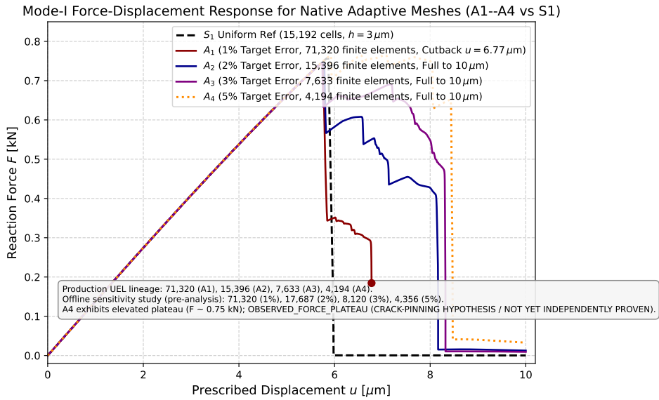
Figure 7.4: Force-displacement curves for native adaptive cases ( A_1 – A_4 ) alongside baseline S_1 .
