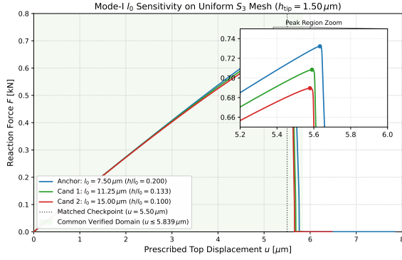
(a) F – u response across l_0
