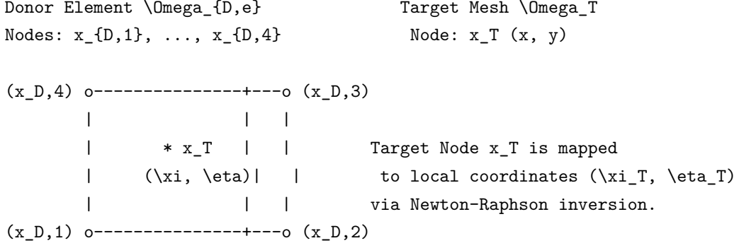
Figure 4.1: Schematic of inverse isoparametric mapping from donor element to target node.
