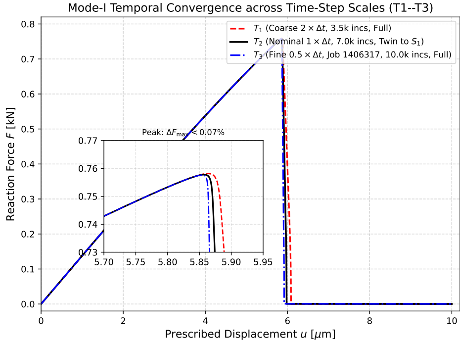
Figure 7.3: Mode-I temporal convergence across time increment scales ( T_1 : 2\times , T_2 : 1\times , T_3 : 0.5\times , Job 1406317.mm.master02), showing step-size invariance of the mechanical peak.
