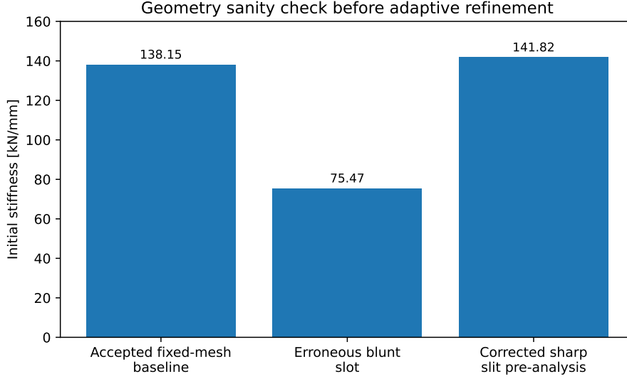
Figure 2.2: Early geometry-sanity-check comparison of structural stiffness K_0 : uncracked solid ( \approx 138.15 kN/mm), blunt notch introducing artificial compliance ( \approx 75.47 kN/mm), and early sharp seam diagnostic ( \approx 141.82 kN/mm). The final governed canonical S_1 sharp-seam reference stiffness is K_0 = 137.945520 kN/mm (Section 2.5).
