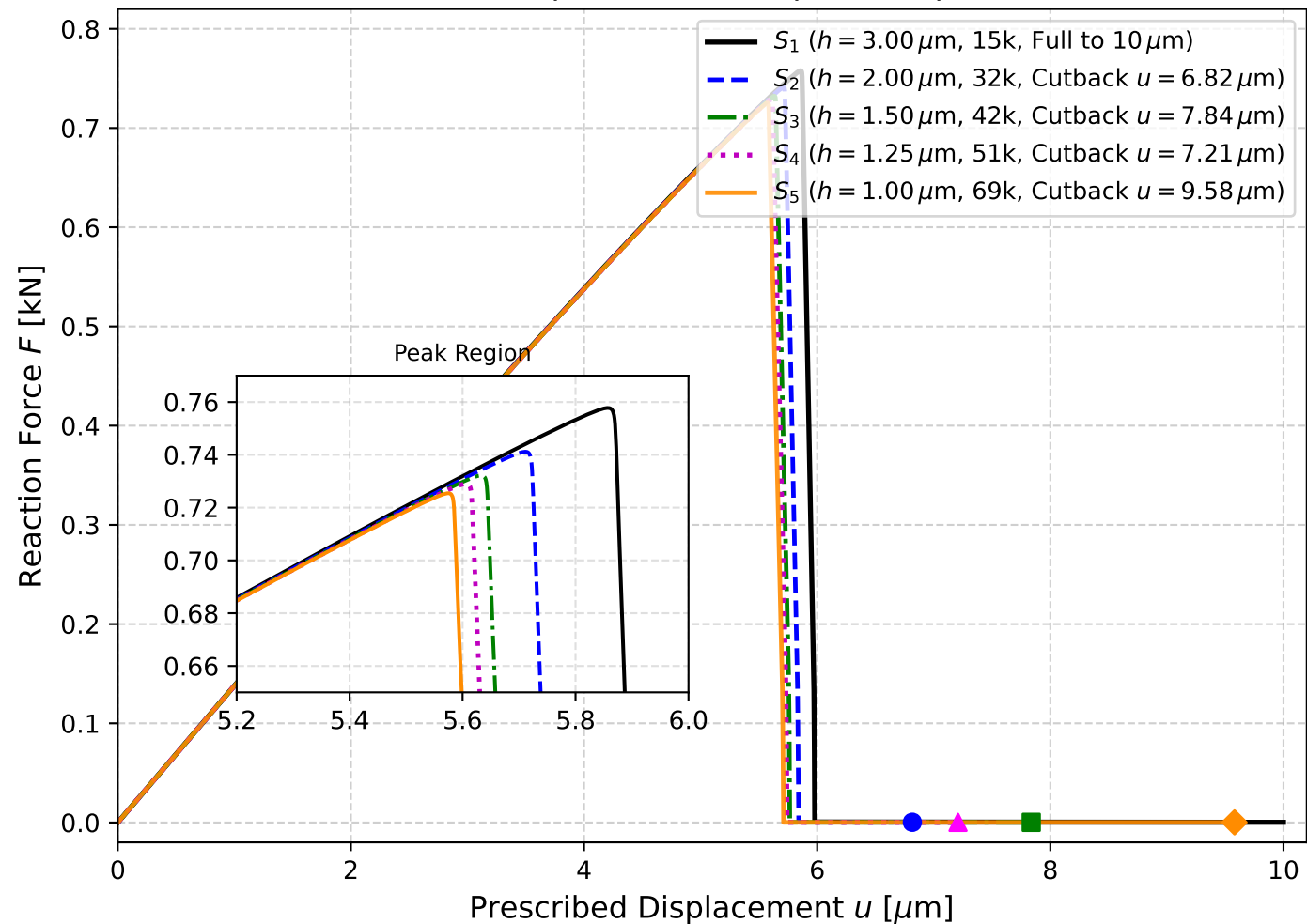
Mode-I Tensile Force-Displacement Response (Spatial Series S1--S5)
