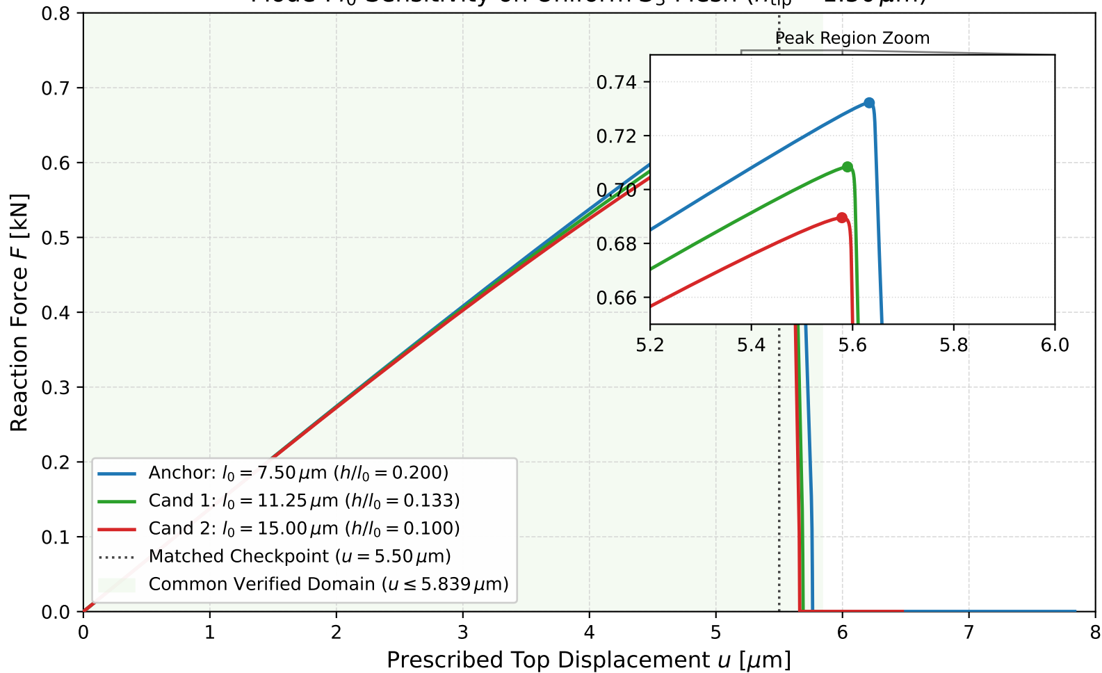
Mode-I l_0 Sensitivity on Uniform S_3 Mesh ( h_{\text{tip}} = 1.50\ \mu\text{m} )
