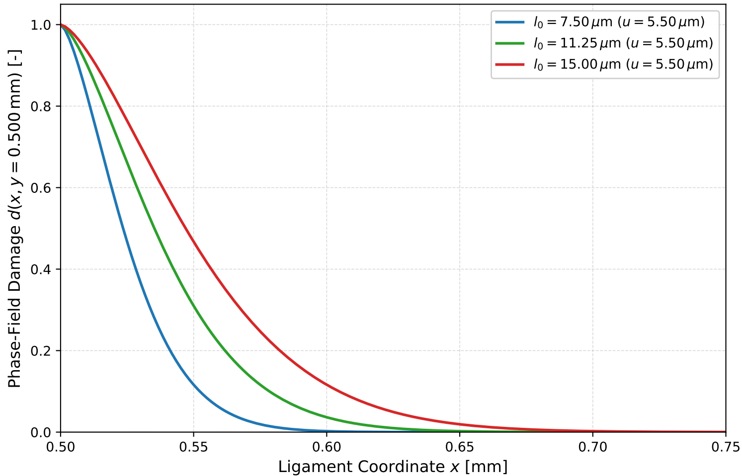
Longitudinal Damage along Zero-Gap Seam ( u = 5.50\text{ }\mu\text{m} )
