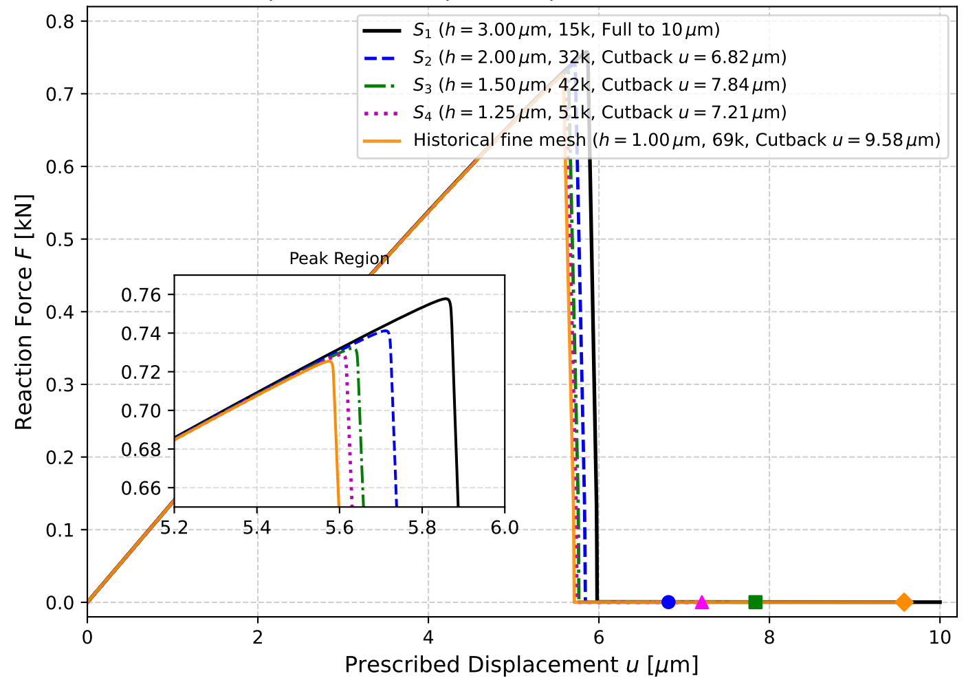
Mode-I Tensile Force-Displacement Response (Spatial Series S1--S4 + Historical Fine Mesh)
