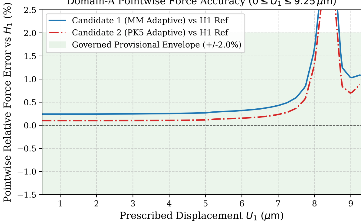
Domain-A Pointwise Force Accuracy ( 0 \leq U_1 \leq 9.25 \mu\text{m} )
