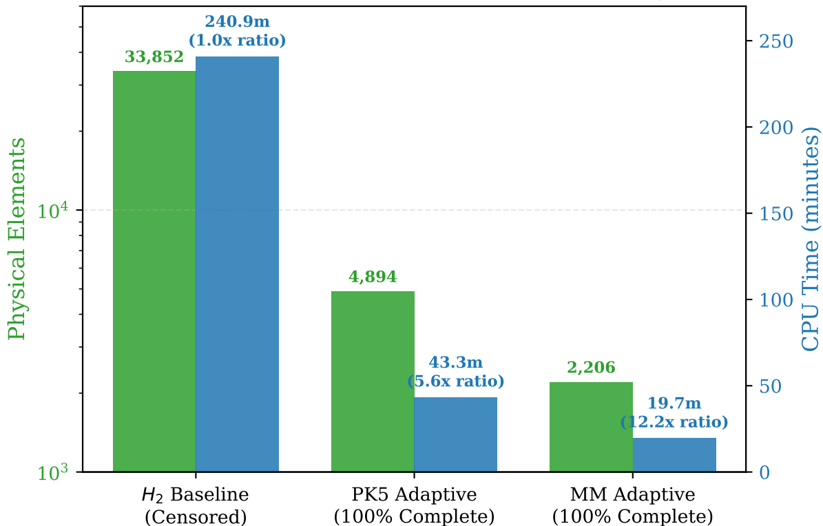
Computational Cost and Mesh Reduction in Stage G
