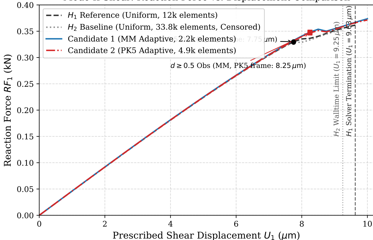
Mode-II Shear: Reaction Force vs. Displacement Comparison
