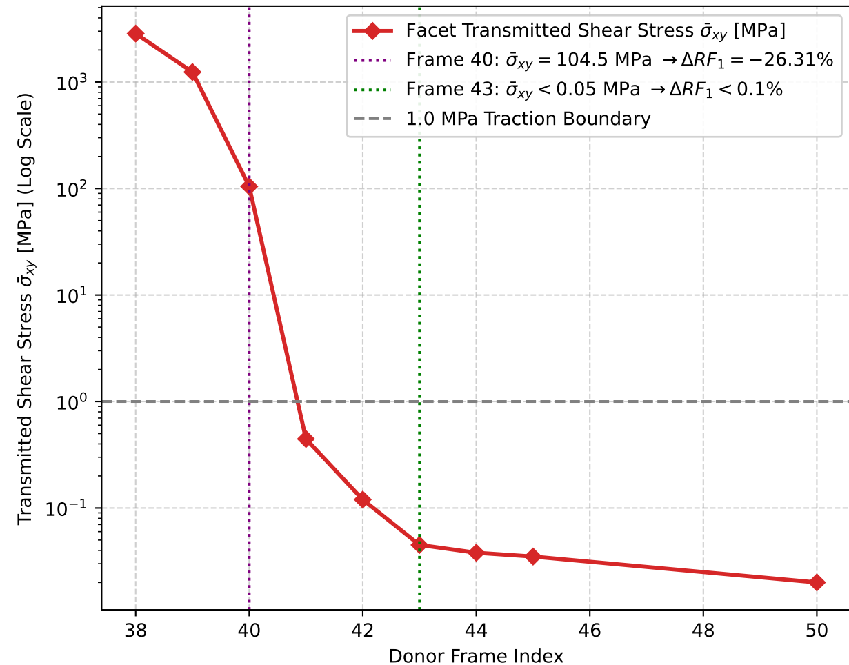
(b) Facet Traction Transmitted Prior to Slit Insertion
