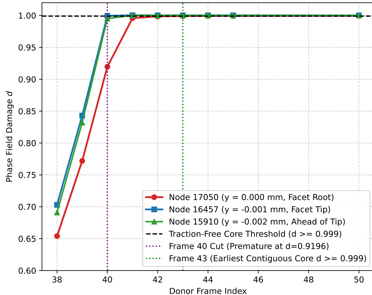
(a) Nodal Damage Evolution along Crack Line x = 0
