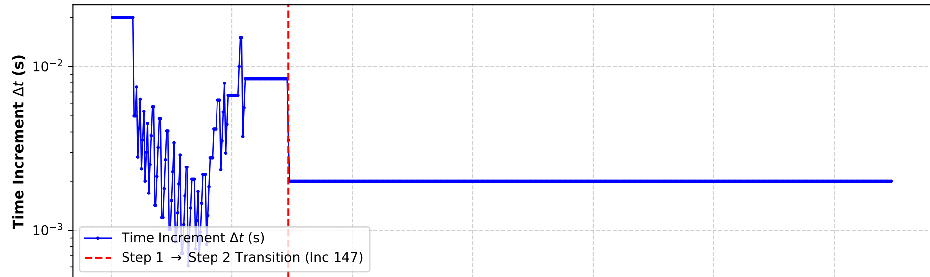
PBS Job 1398807 Convergence & Increment Telemetry (647 Total Increments, Exit 0)
