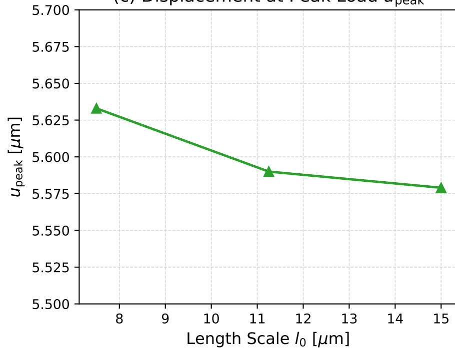
(c) Displacement at Peak Load u_{\text{peak}}
