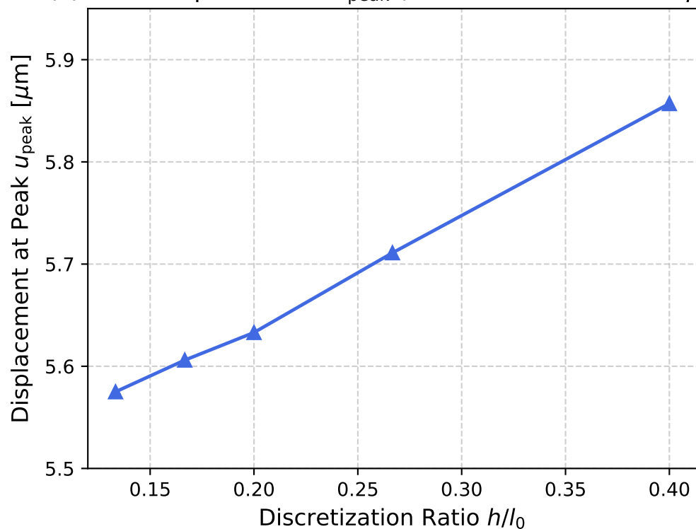
(c) Peak Displacement u_{\text{peak}} (Decreases 5.86 \rightarrow 5.58 \mu\text{m} )
