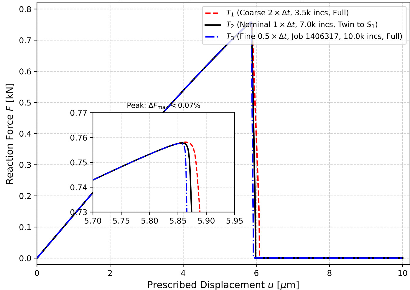
Mode-I Temporal Convergence across Time-Step Scales (T1--T3)
