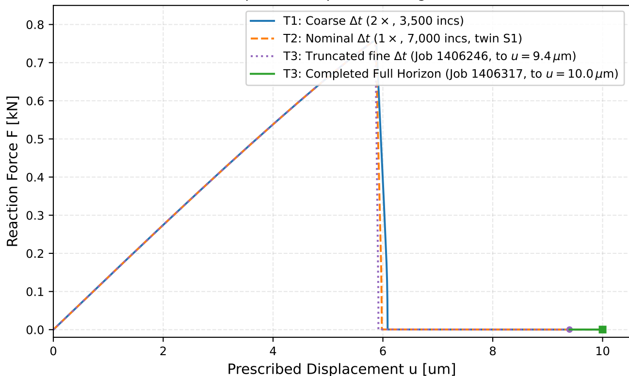
Mode-I Tensile Response: Temporal Convergence Series (T1--T3)
