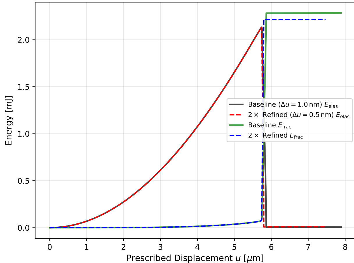
2 × Temporal Refinement Energy Evolution (8,958 Incs)
