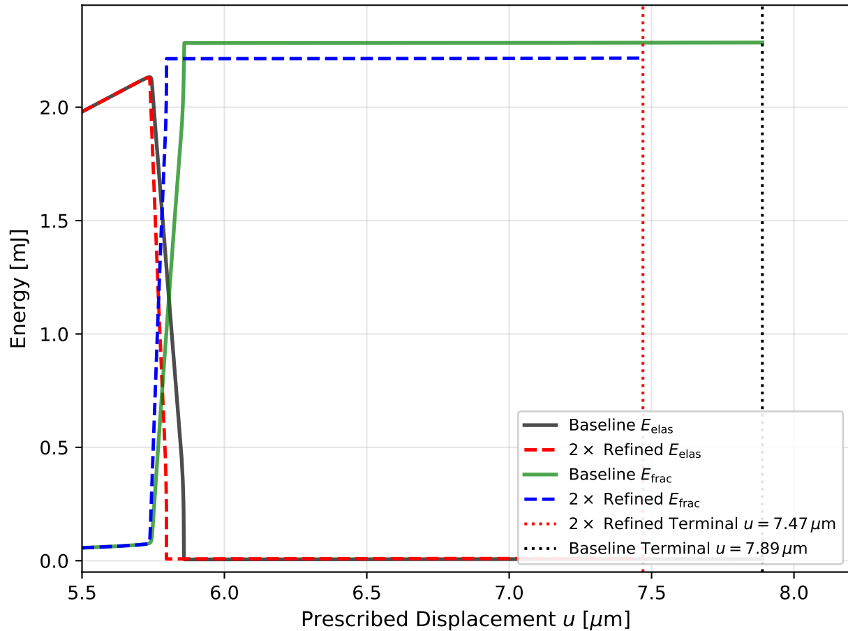
Fracture & Post-Fracture Softening Regime Detail
