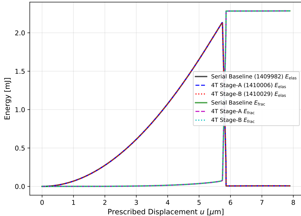
4-Thread Shared-Memory Energy Determinism (4,890 Incs)
