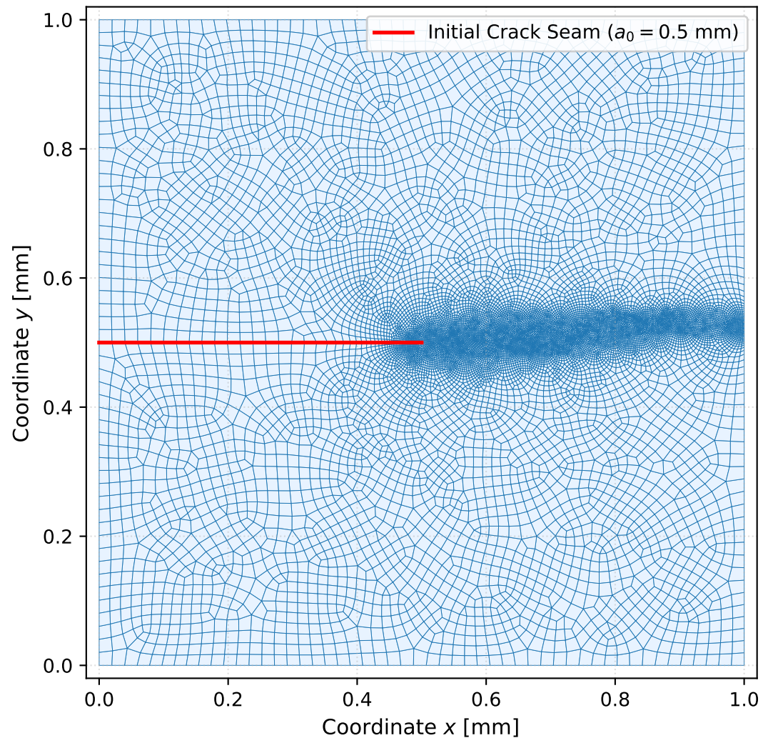
Native Abaqus Adaptive Mesh (Stage 14) 14,483 Elements (14,082 Quads + 401 Tris), 14,456 Nodes
