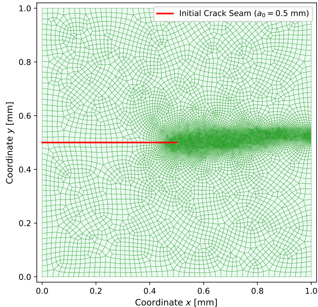
Reconstructed Stage-14 Underlying Mesh (Job 1409947) 14,483 Base Elements (43,449 3-Layer Elements)
