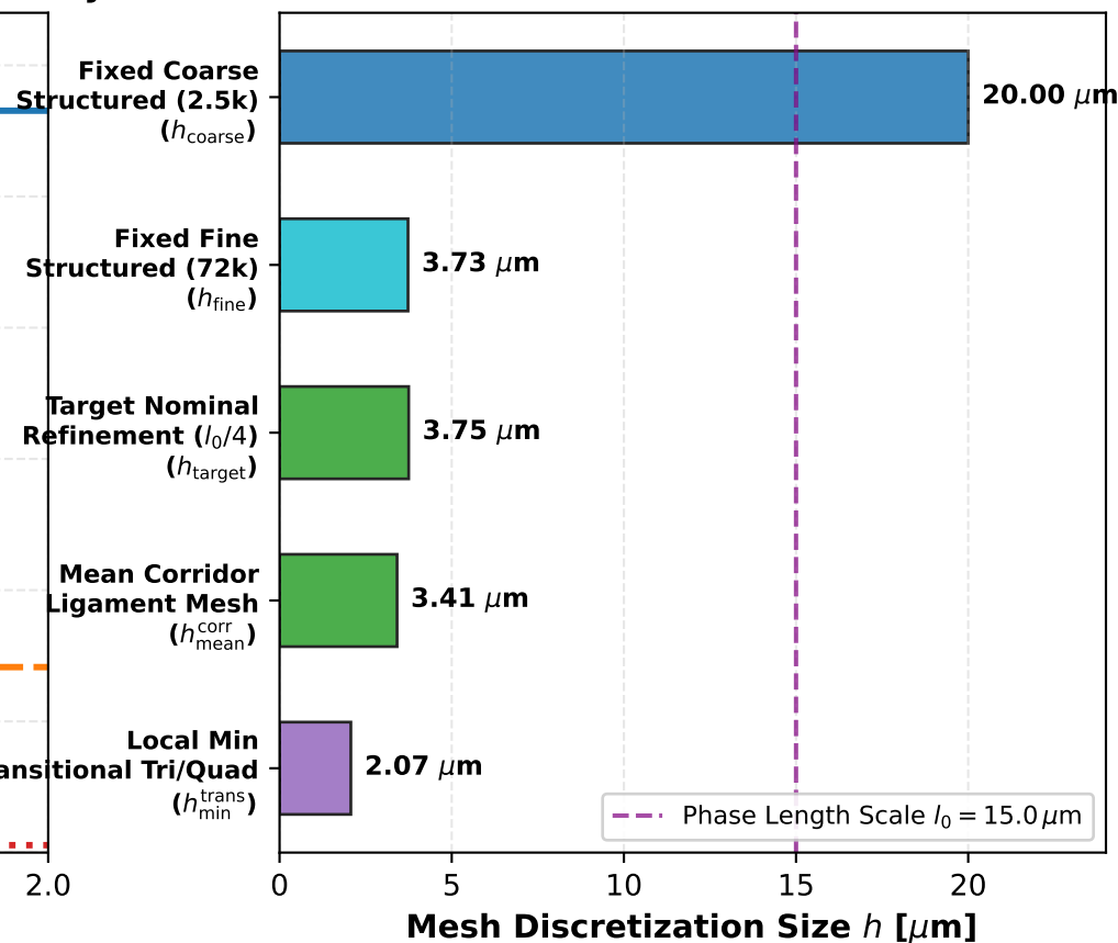
(e) Discretization Metrics & h_{\min} Reconciliation
