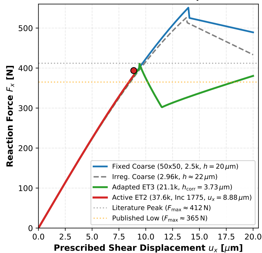
(a) Full Monotonic Mode-II Response ( F - u )
