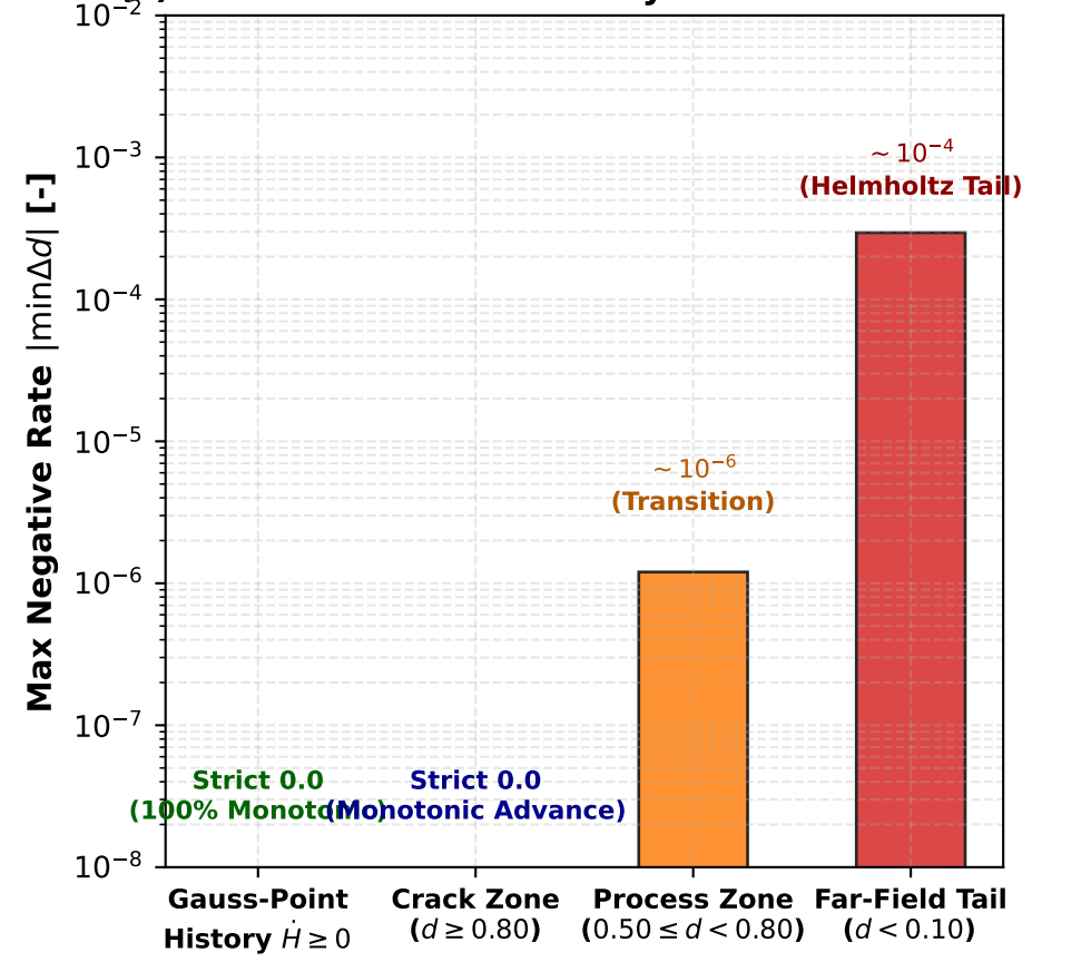
(c) Pointwise Irreversibility &amp; Tail Fluctuations
