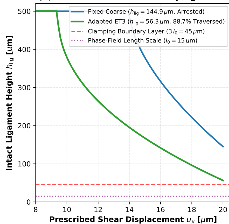
(b) Crack Penetration &amp; Clamping Arrest
