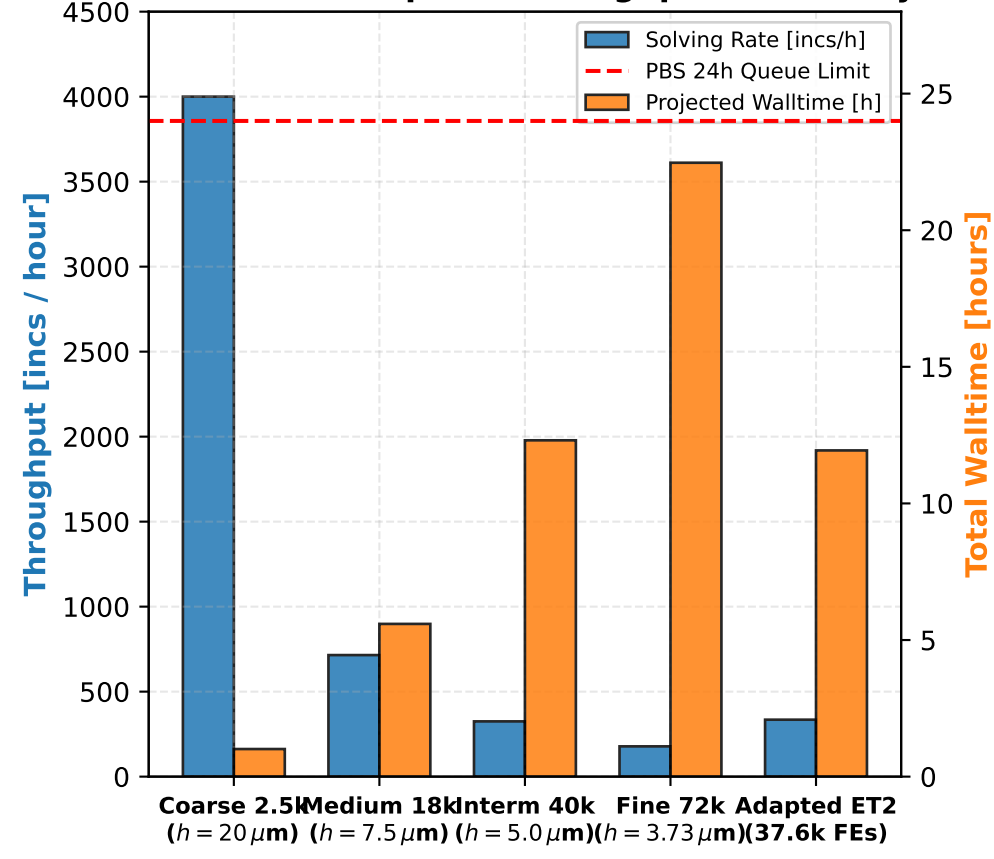
(f) Fixed &amp; Adaptive Throughput Feasibility
