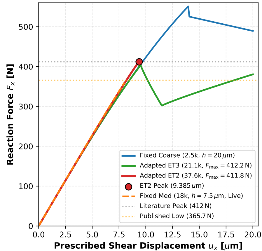
(a) Multi-Discretization Mode-II Response
