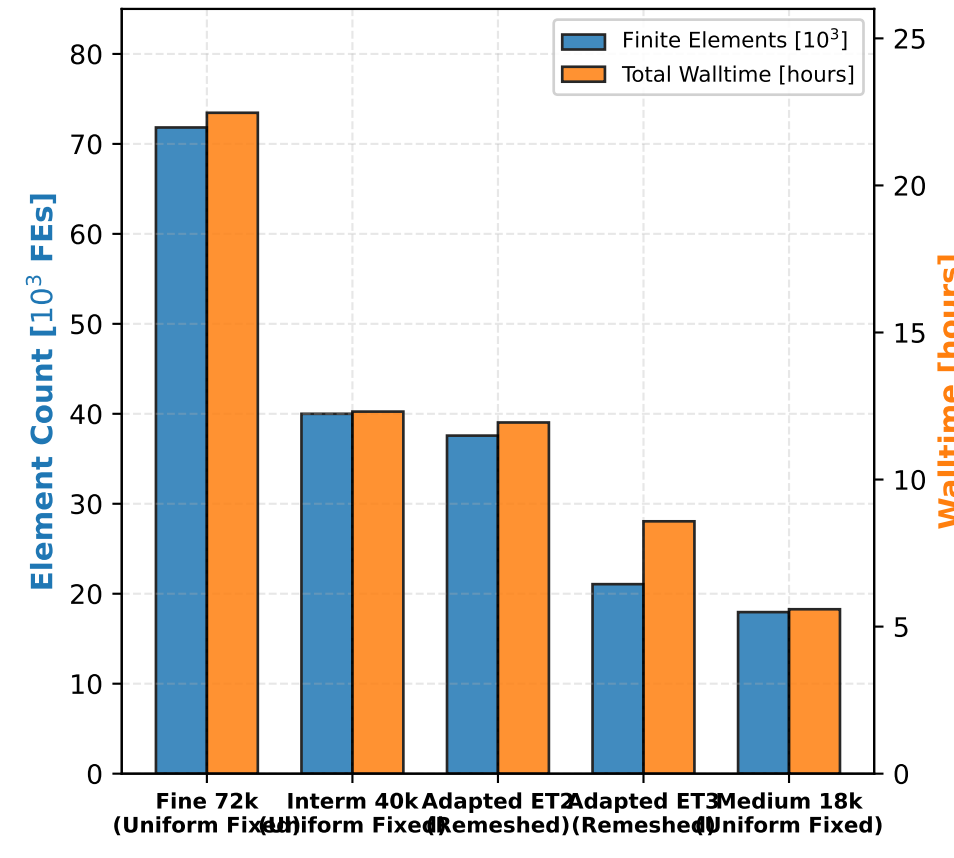
(f) Computational Economy &amp; Walltime
