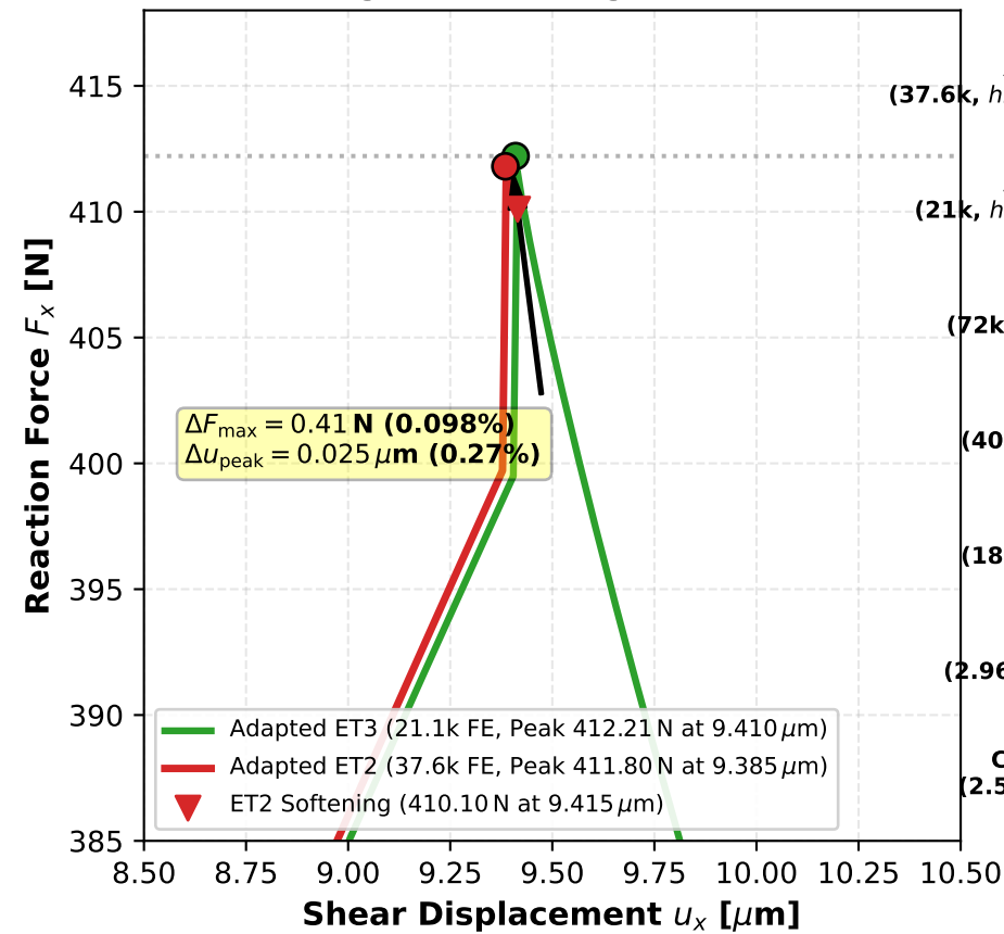
(b) Peak Regime Convergence (ET2 vs ET3)
