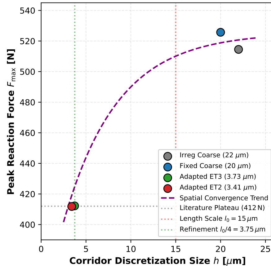
(e) Peak Load vs Spatial Discretization ( h )
