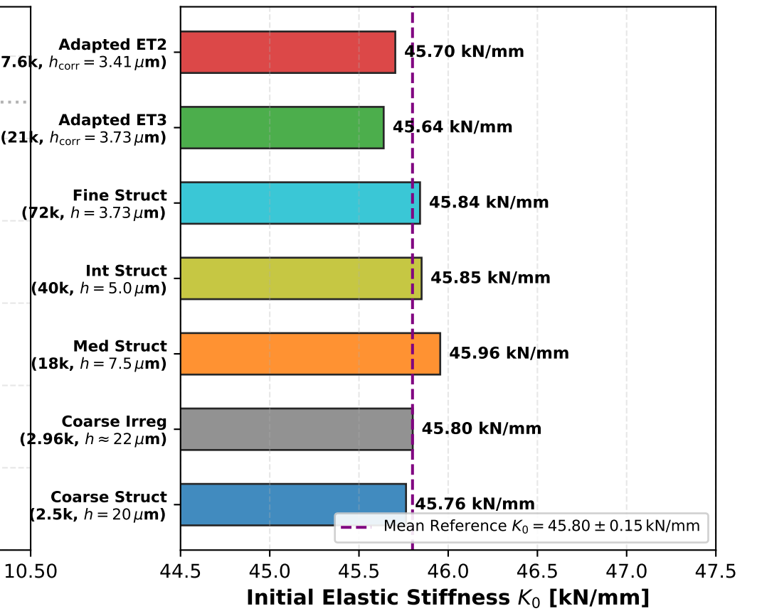
(c) Elastic Stiffness Invariance (7 Meshes)
