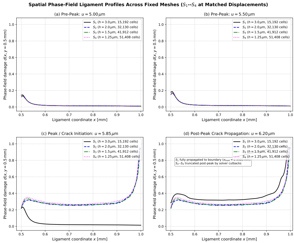
Fig. 4.11.: Spatial phase-field ligament profiles d(x, y = 0.5 \text{ mm}) for fixed meshes S_1 – S_4 across matched displacement levels, showing x-axis coordinates on all panels and annotating full boundary propagation in S_1 at u = 6.20 \mu\text{m} .
