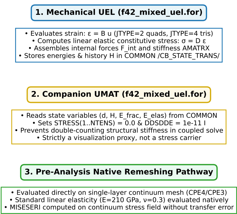
(a) UEL/UMAT Architecture & Stress Pathway
