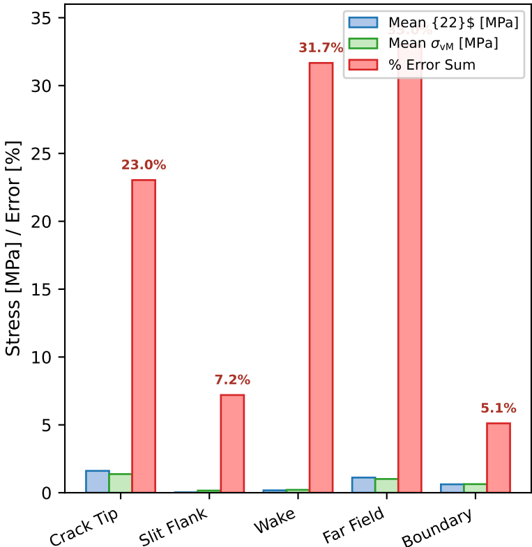
(e) 5-Region Stress & Error Breakdown
