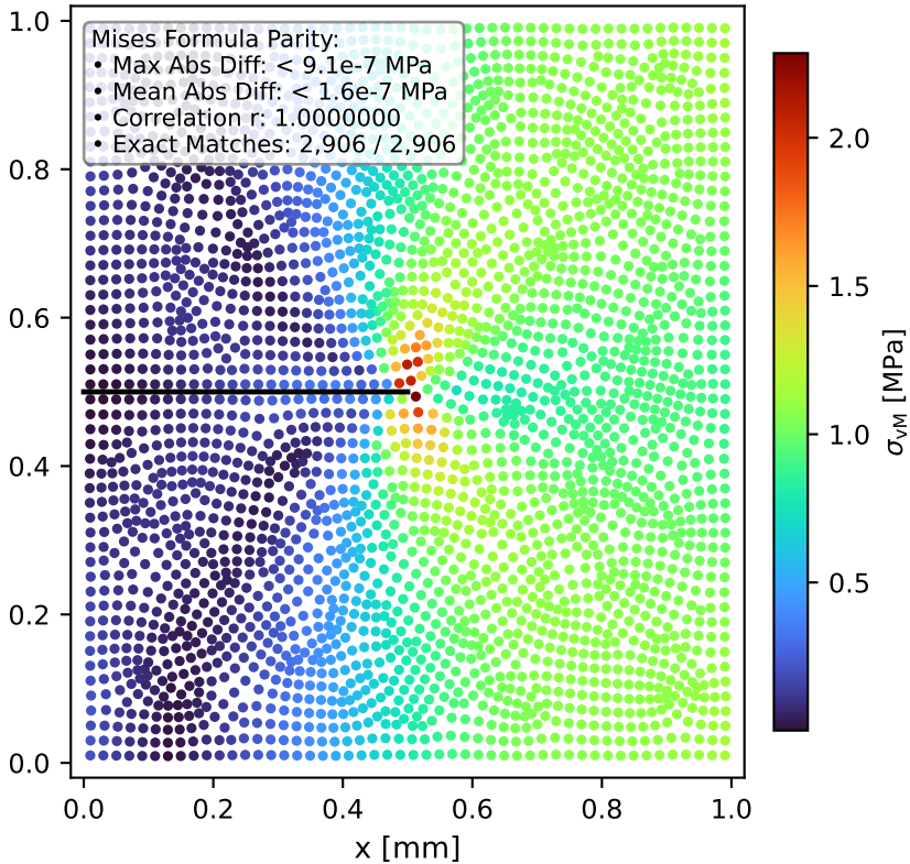
(c) Equivalent Mises Stress \sigma_{VM} [MPa]
