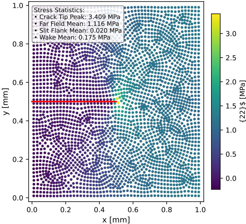
(b) Tensile Stress Field {22}$ [MPa]
