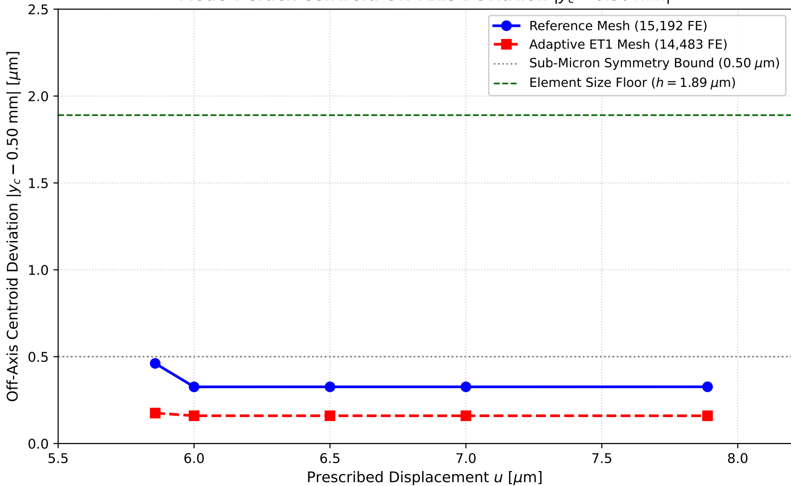
Mode-I Crack Centroid Off-Axis Deviation |y_c - 0.50 \text{ mm}|
