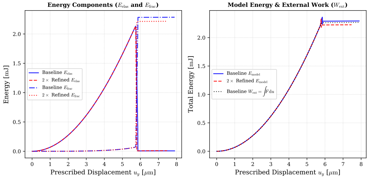
Figure 14: Matched energy evolution for baseline and 2 \times temporal refined models: (a) stored elastic energy E_{\text{elas}} and fracture functional E_{\text{frac}} ; (b) total model energy E_{\text{model}} and external work W_{\text{ext}} .
