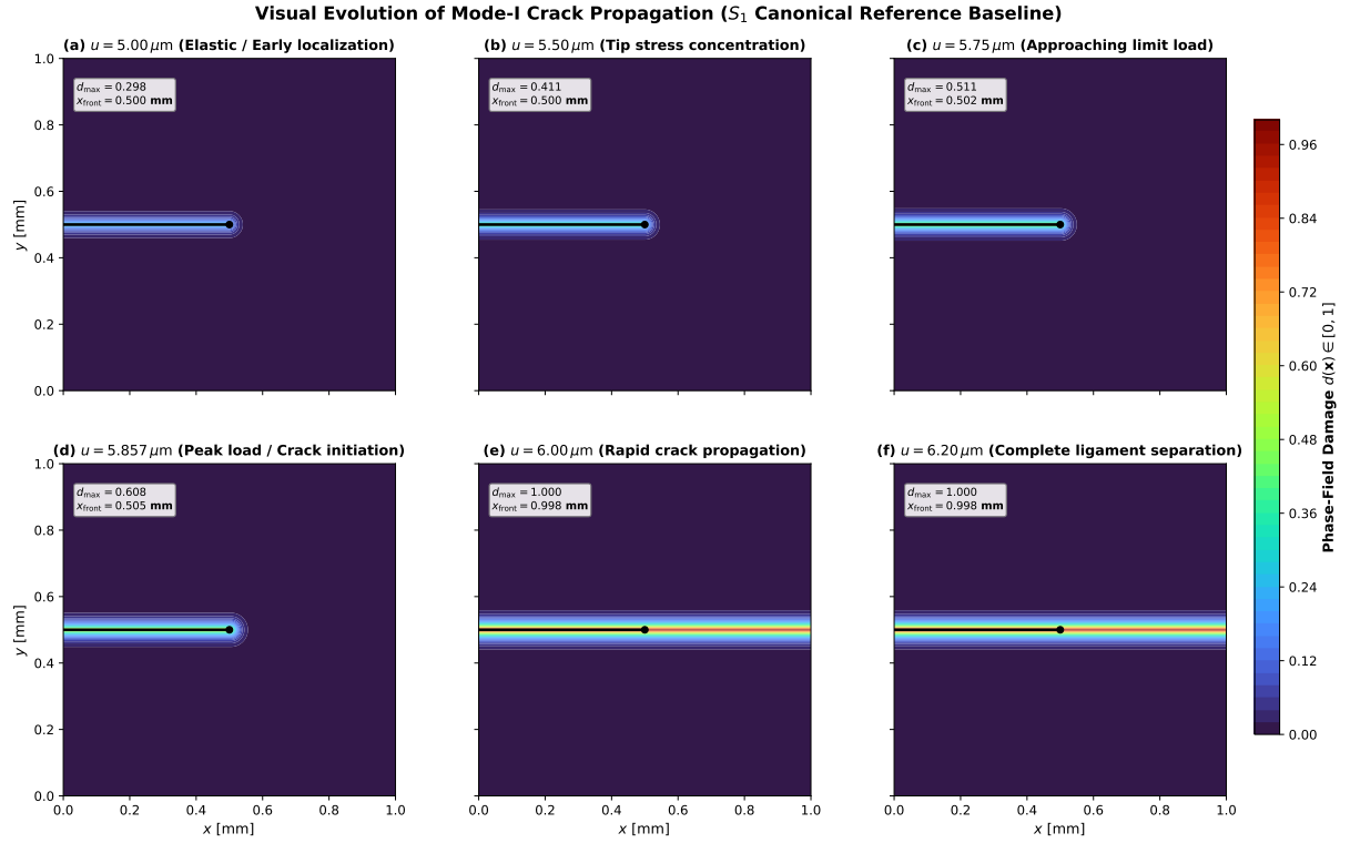
Figure 24: Visual evolution of Mode-I crack propagation for the canonical S_1 reference baseline: six-stage sequence from initial elastic localization ( u = 5.0 \mu\text{m} ) through peak load ( u = 5.857 \mu\text{m} ) to complete ligament separation ( u = 6.20 \mu\text{m} ).
