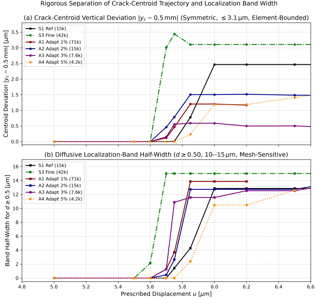
Figure 25: Rigorous separation of (a) damage-weighted crack-centroid offset versus prescribed displacement ( |y_c - 0.5| \leq 3.1 \mu\text{m} , symmetric) and (b) damage localization-band half-width (10–15 \mu\text{m} , resolution-limited).
