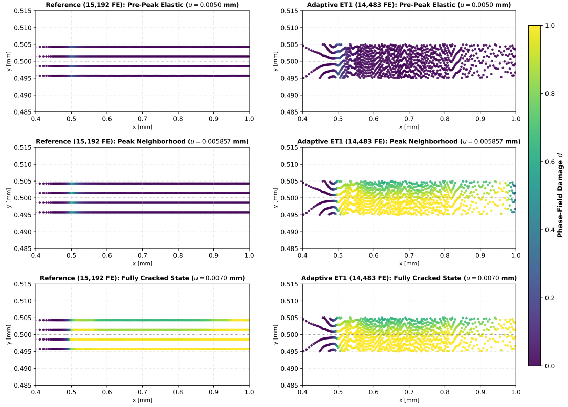
Figure 17: Two-dimensional phase-field damage contour comparison d(x, y) between Fixed Reference (15,192 FE) and Adaptive ET1 (14,483 FE) at matched deformation states: u = 5.0 \mu\text{m} , u = 5.857 \mu\text{m} , and u = 7.0 \mu\text{m} .
