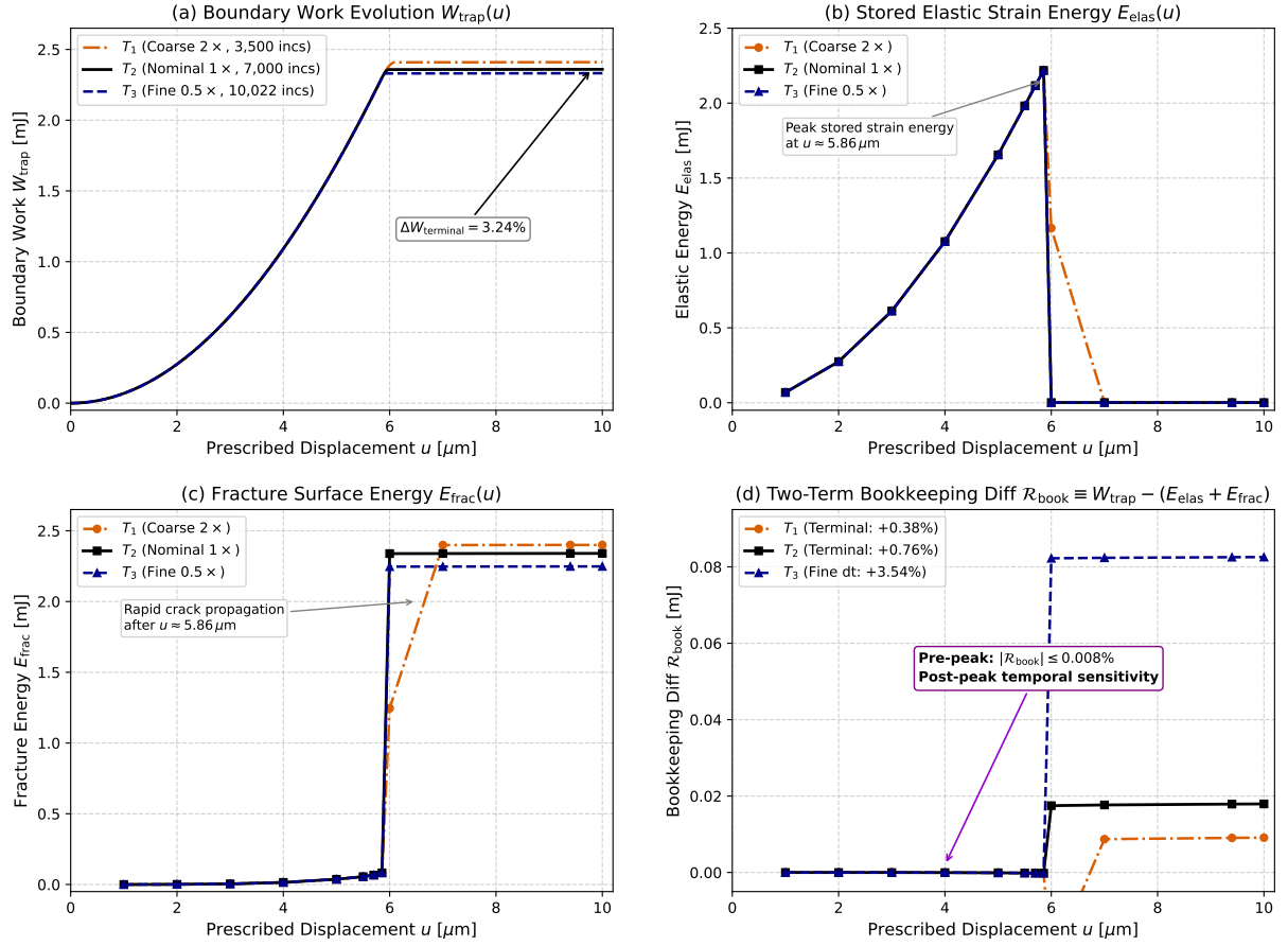
Figure 28: Temporal discretization scaling of global energy components across schedules T_1 ( 2 \times ), T_2 ( 1 \times ), and T_3 ( 0.5 \times , Job 1406317) on fixed S_1 mesh: (a) boundary work W_{\text{trap}}(u) ; (b) stored elastic energy E_{\text{elas}}(u) ; (c) fracture surface energy E_{\text{frac}}(u) ; (d) two-term bookkeeping difference \Delta_{\text{book}}(u) .
