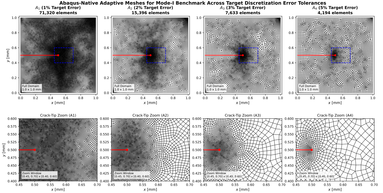
Figure 19: Abaqus-native adaptive meshes generated for the Mode-I benchmark using errorTarget values of (a) 1%, (b) 2%, (c) 3%, and (d) 5%. The corresponding production meshes contain 71,320, 15,396, 7,633, and 4,194 underlying finite elements, respectively. Full-domain views and identical crack-tip zooms illustrate how relaxing the target error changes the spatial refinement distribution.
