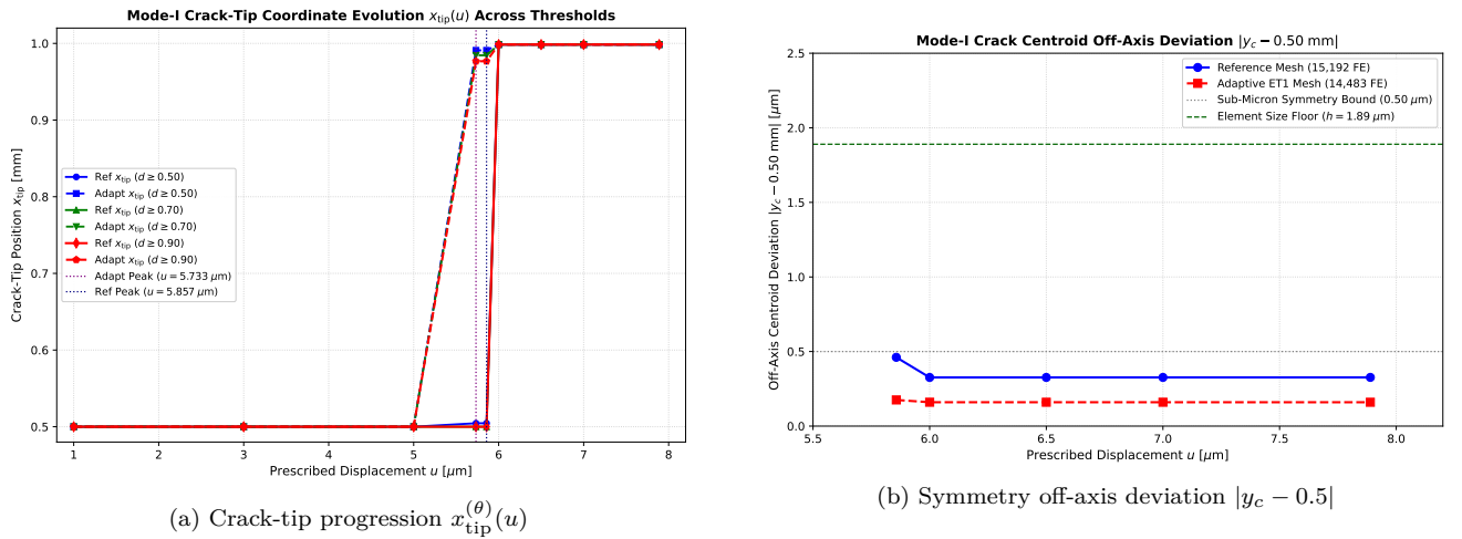
Figure 18: Crack propagation kinematics: (a) crack-tip coordinate x_{\text{tip}}^{(\theta)} for thresholds \theta \in \{0.50, 0.70, 0.90\} ; (b) damage centroid off-axis deviation showing sub-micron symmetry preservation ( < 0.5 \mu\text{m} ).
