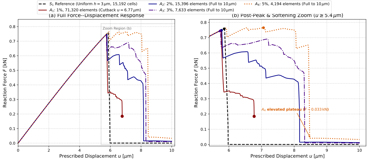
Figure 20: Force–displacement response of the canonical uniform reference S_1 and native adaptive meshes A_1 – A_4 : (a) full response over u \in [0, 10] \mu\text{m} ; (b) post-peak zoom over u \in [5.4, 10] \mu\text{m} . Production adaptive meshes contain 71,320, 15,396, 7,633, and 4,194 underlying finite elements for errorTarget values of 1%, 2%, 3%, and 5%, respectively. A_1 terminates at u = 6.77 \mu\text{m} , whereas A_2 – A_4 reach 10 \mu\text{m} .
