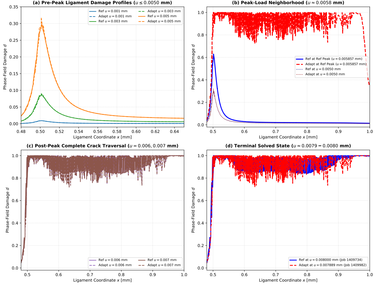
Figure 16: Matched-displacement phase-field ligament profiles d(x, y = 0.5 mm) comparing Fixed Reference (15,192 FE) and Adaptive ET1 (14,483 FE) across (a) pre-peak elastic, (b) peak-neighborhood, (c) post-fracture, and (d) terminal states.
