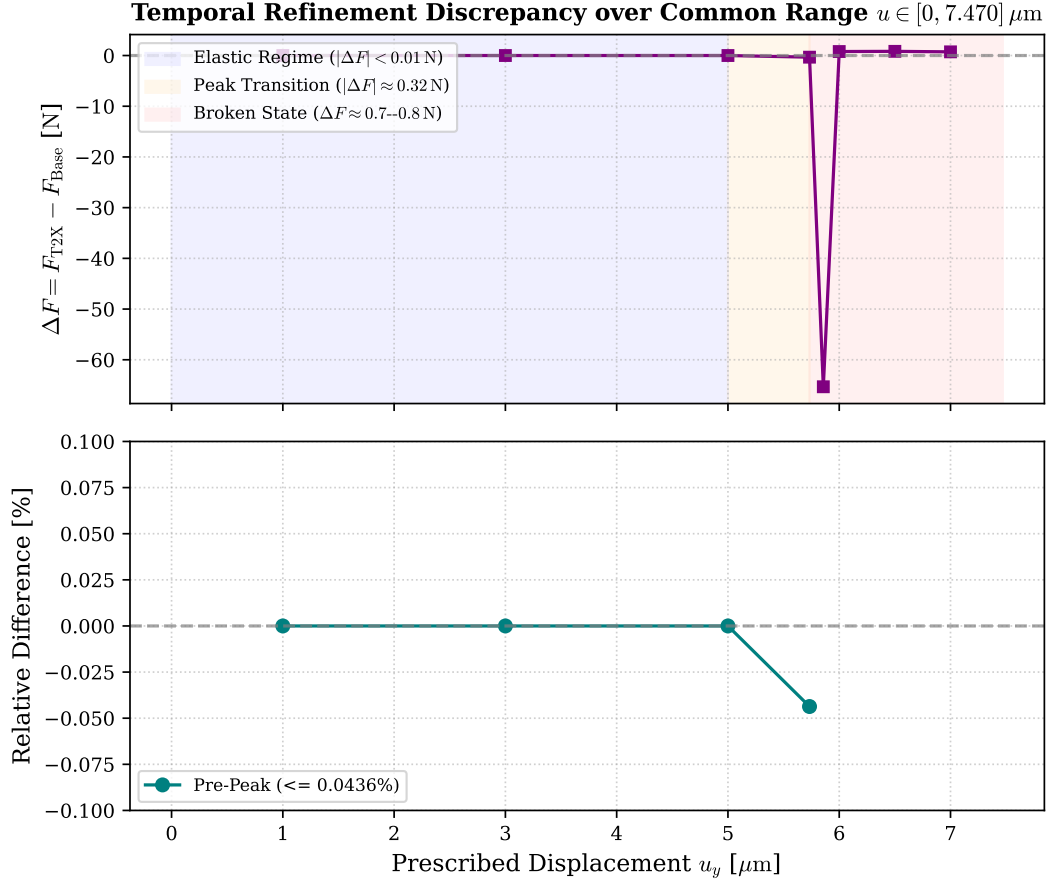
Figure 13: Pointwise force discrepancy \Delta F and relative difference [%] over the common reached displacement interval u \in [0, 7.470] \mu\text{m} , separating elastic ( \leq 0.0436\% ) from post-peak broken-state regimes.
