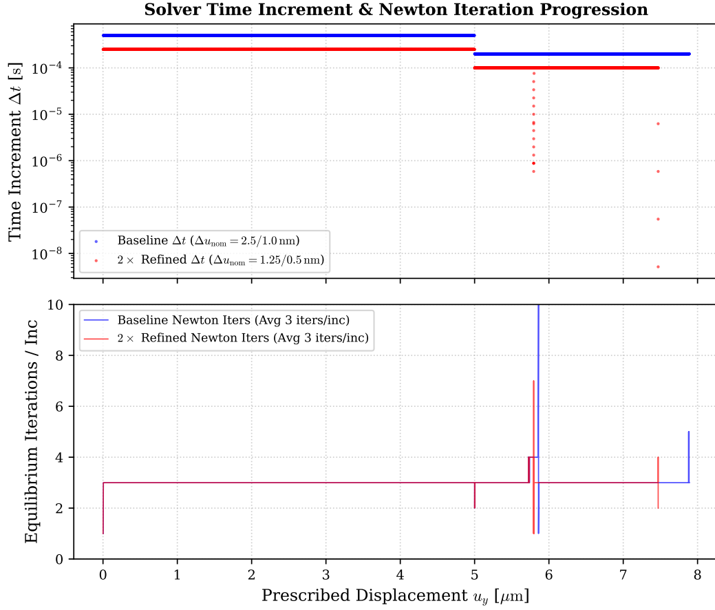
Figure 15: Solver time increment \Delta t progression (log scale) and Newton equilibrium iterations per increment across baseline and 2 \times refined runs, showing consistent 3 iters/inc across all reached states.
