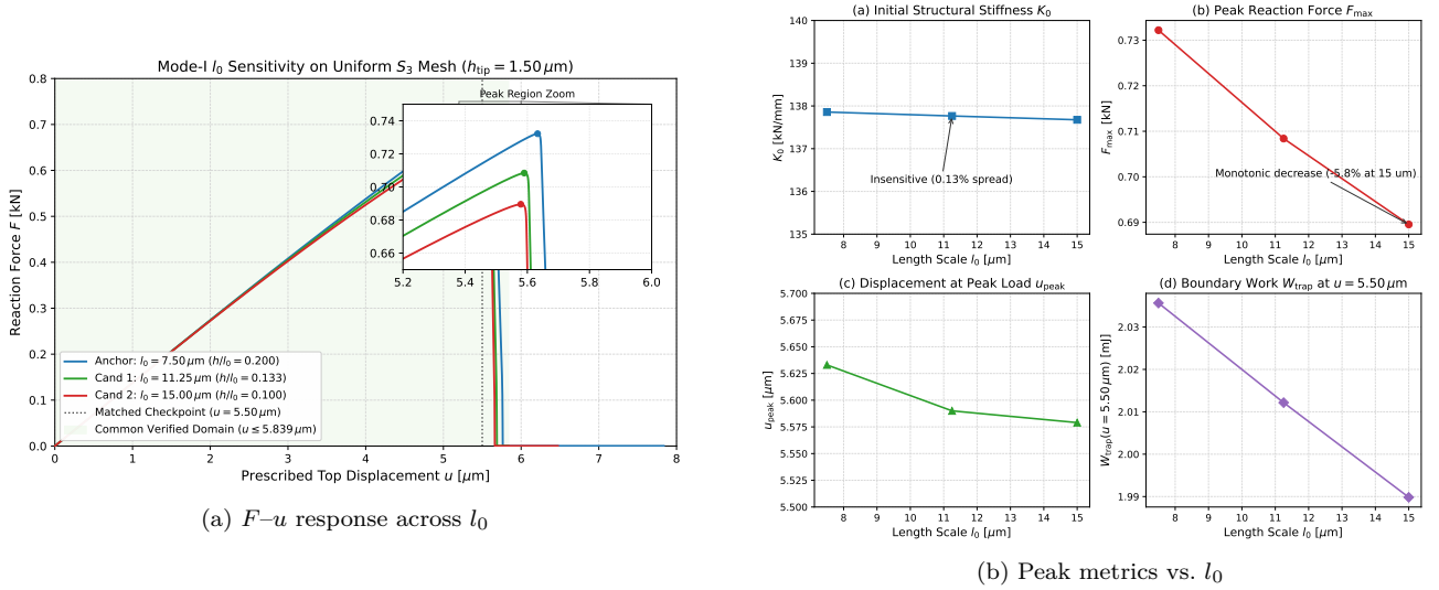
Figure 26: Three-point physical length-scale study on fixed S_3 mesh ( h = 1.5 \mu\text{m} ): (a) global force-displacement overlay and (b) variation of K_0 , F_{\max} , u_{\text{peak}} , and matched W_{\text{trap}} at u = 5.50 \mu\text{m} with l_0 .
