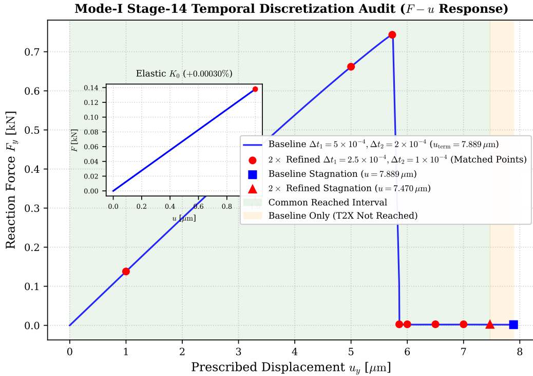
Figure 12: Mode-I adaptive mesh 2× temporal refinement audit: F-u response comparing Baseline (4,890 incs, u_{\text{term}} = 7.889 \mu\text{m} ) against 2× Refined (8,958 incs, u_{\text{term}} = 7.470 \mu\text{m} ), highlighting common reached interval and pre-peak K_0 inset.
