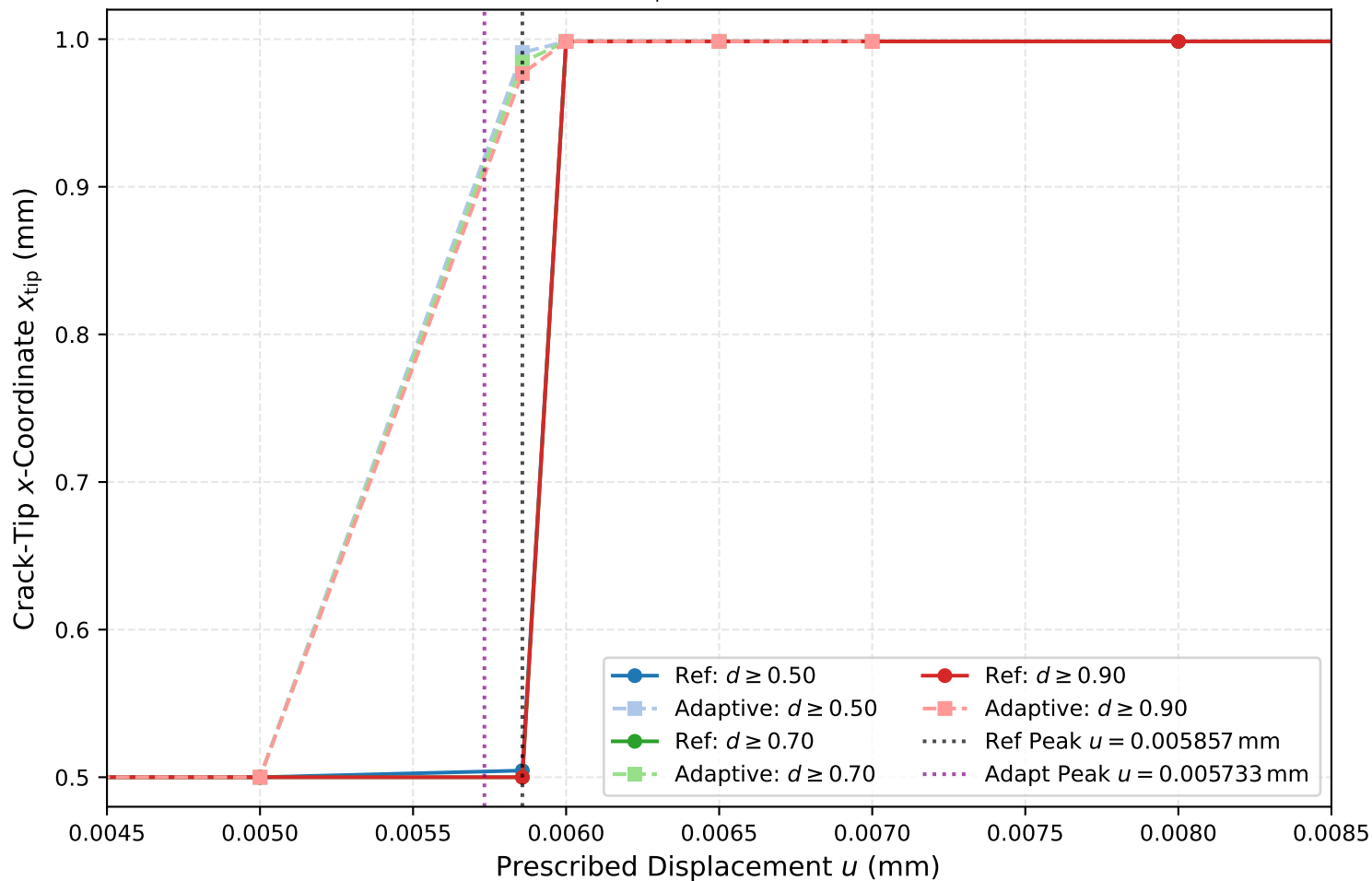
Crack-Tip Position Evolution x_{\text{tip}}(u) across Multiple Damage Thresholds
