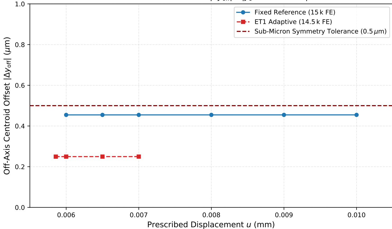
Phase-Field Centroid Off-Axis Deviation |\Delta y_{\text{off}}| = |y_c - 0.5000 \text{ mm}| at x = 0.75 \text{ mm}
