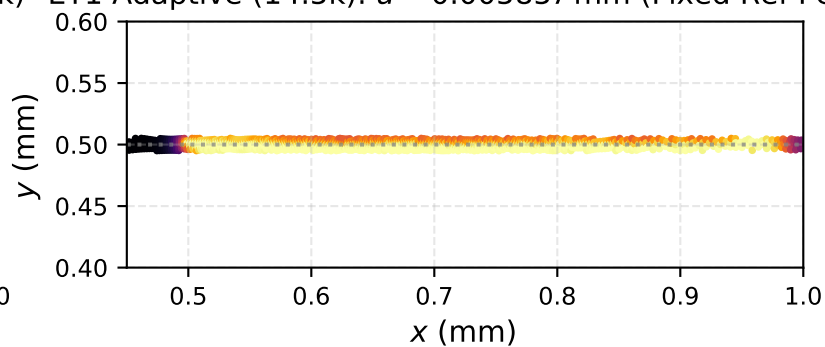
ET1 Adaptive (14.5k): u = 0.005857 mm (Fixed Ref Peak)
