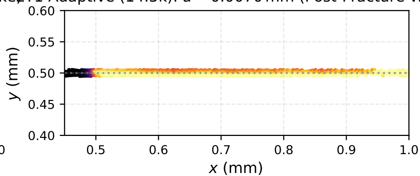
ET1 Adaptive (14.5k): u = 0.0070 mm (Post-Fracture Wake)
