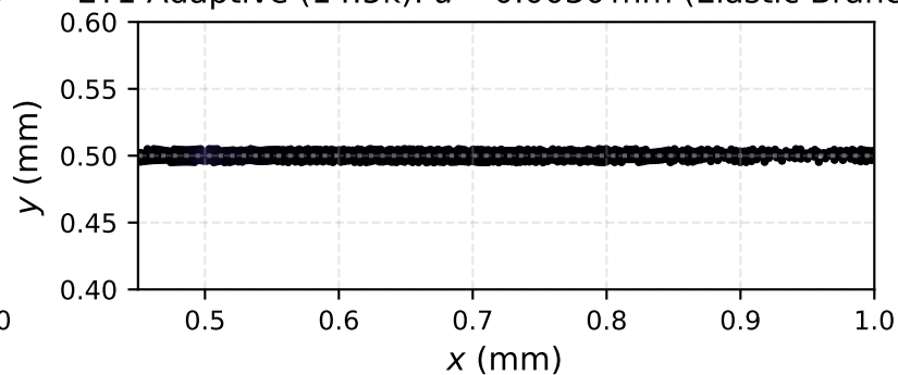
ET1 Adaptive (14.5k): u = 0.0030 mm (Elastic Branch)
