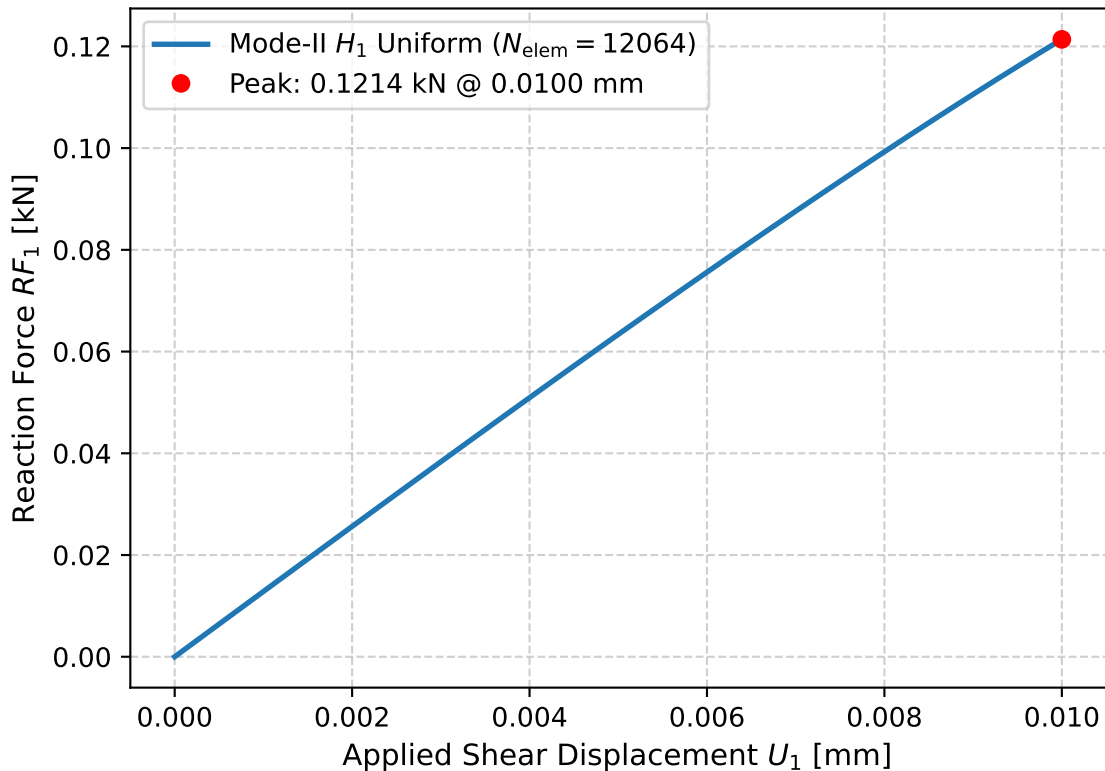
Mode-II Pure Shear Reference Response ( H_1 Uniform)
