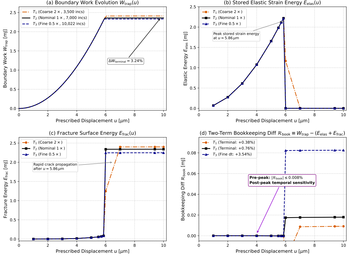
Figure 21: Temporal discretization scaling of global energy components across schedules T_1 ( 2 \times ), T_2 ( 1 \times ), and T_3 ( 0.5 \times , Job 1406317) on fixed S_1 mesh: (a) boundary work W_{\text{trap}}(u) ; (b) stored elastic energy E_{\text{elas}}(u) ; (c) fracture surface energy E_{\text{frac}}(u) ; (d) two-term bookkeeping difference \Delta_{\text{book}}(u) .
